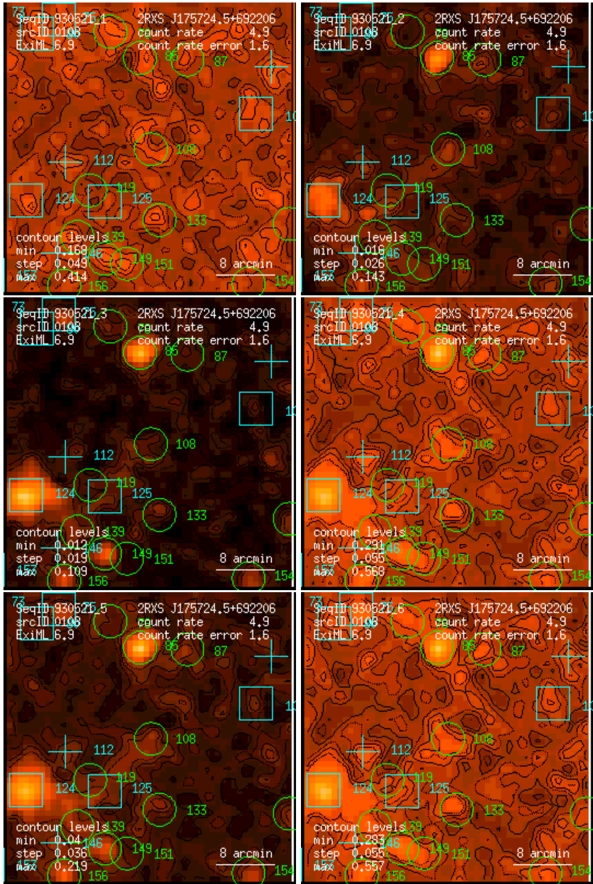
Figure 108: RASS 930521: detection 0108: band rate images, Gaussian filter: (1) PSPC channels 11 – 41, (2) 52 – 90, (3) 91 – 201, (4) 11 – 235, (5) 52 – 201, (6) 11 – 201. Broad band rates in counts/ks. Band rate contour levels in counts/ks/arcmin 2 .
