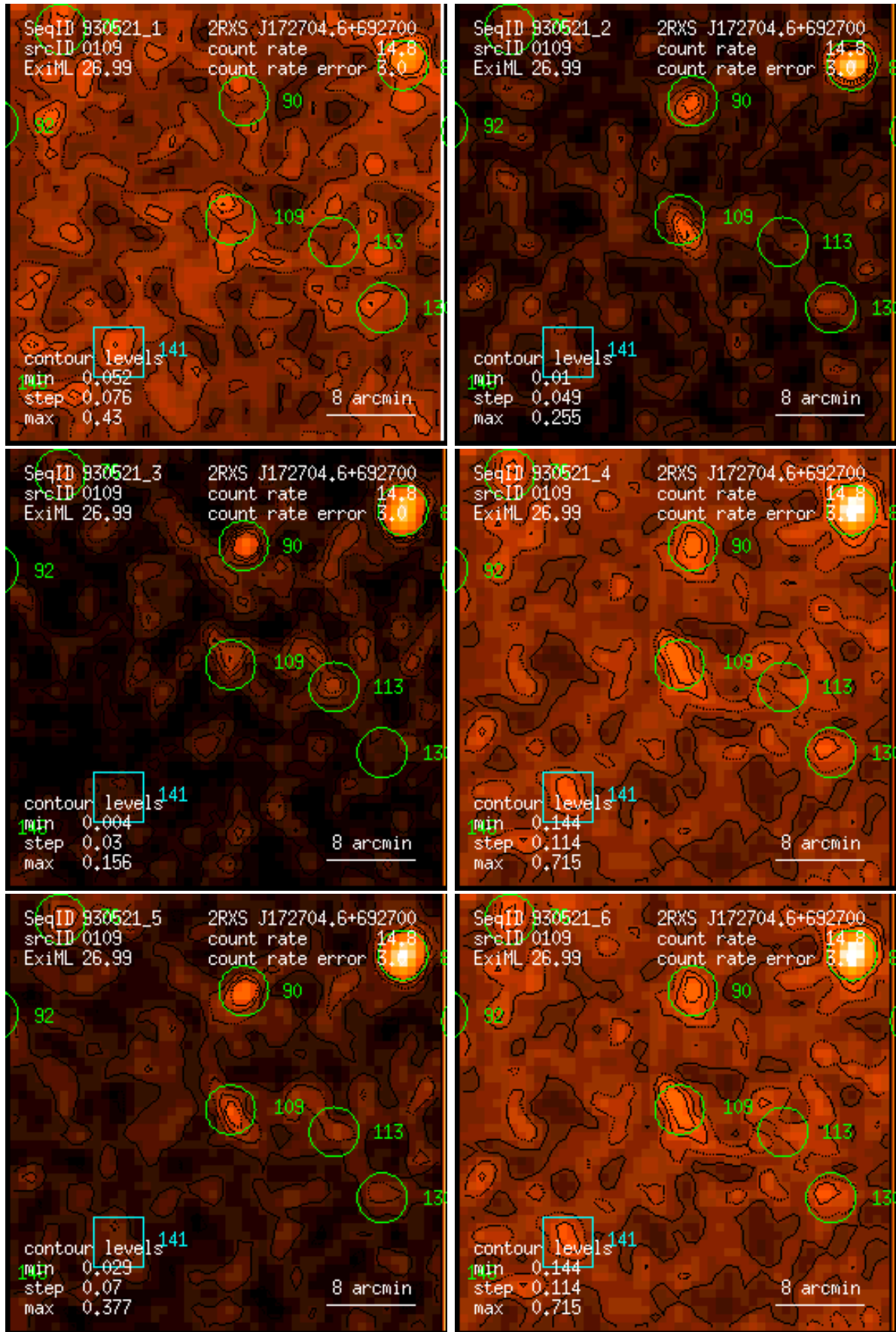
Figure 109: RASS 930521: detection 0109: band rate images, Gaussian filter: (1) PSPC channels 11 – 41, (2) 52 – 90, (3) 91 – 201, (4) 11 – 235, (5) 52 – 201, (6) 11 – 201. Broad band rates in counts/ks. Band rate contour levels in counts/ks/arcmin 2 .
