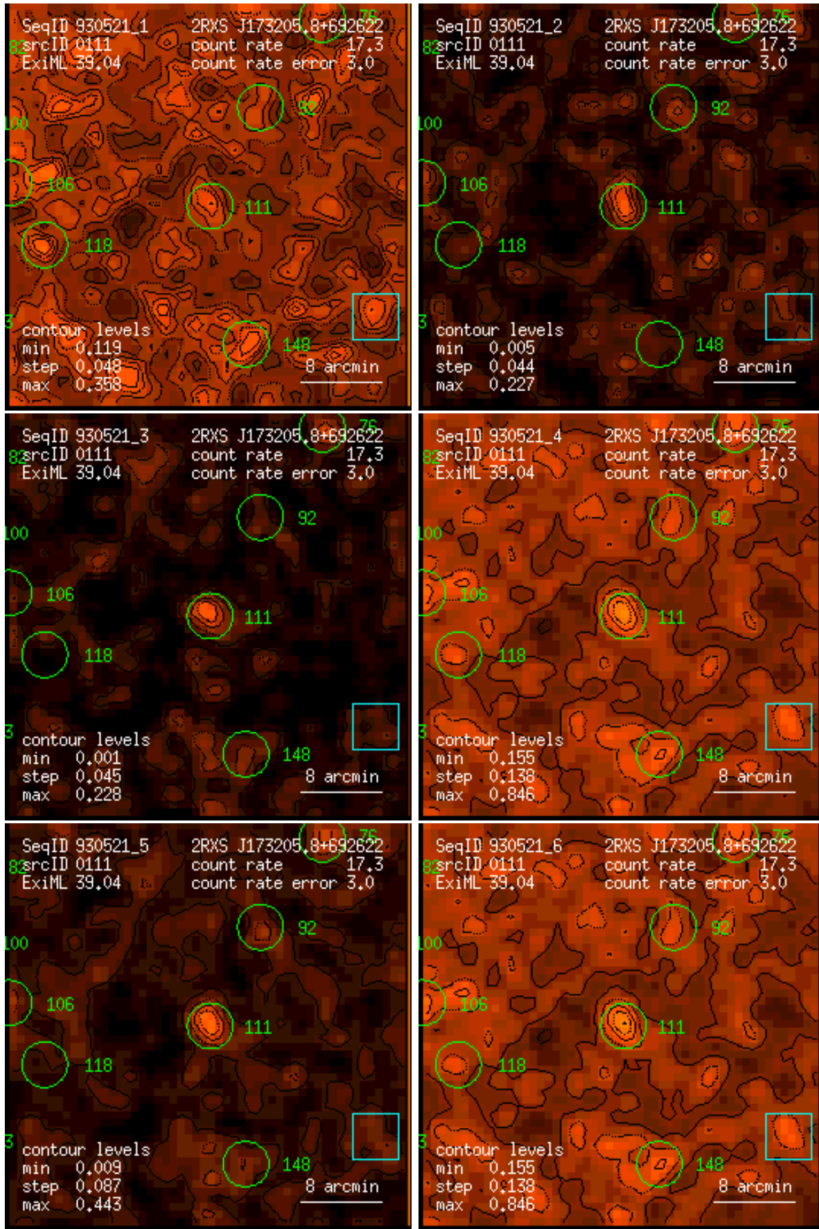
Figure 111: RASS 930521: detection 0111: band rate images, Gaussian filter: (1) PSPC channels 11 – 41, (2) 52 – 90, (3) 91 – 201, (4) 11 – 235, (5) 52 – 201, (6) 11 – 201. Broad band rates in counts/ks. Band rate contour levels in counts/ks/arcmin 2 .
