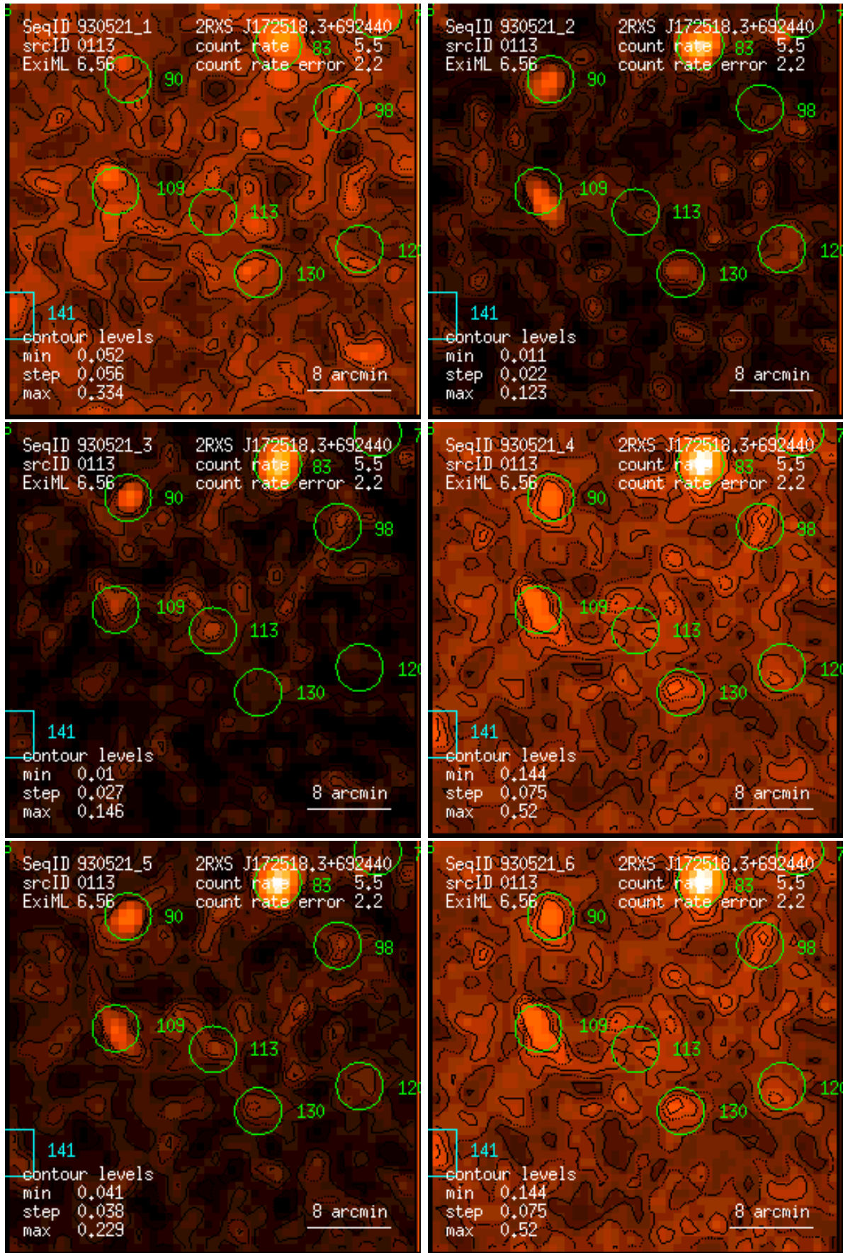
Figure 113: RASS 930521: detection 0113: band rate images, Gaussian filter: (1) PSPC channels 11 – 41, (2) 52 – 90, (3) 91 – 201, (4) 11 – 235, (5) 52 – 201, (6) 11 – 201. Broad band rates in counts/ks. Band rate contour levels in counts/ks/arcmin 2 .
