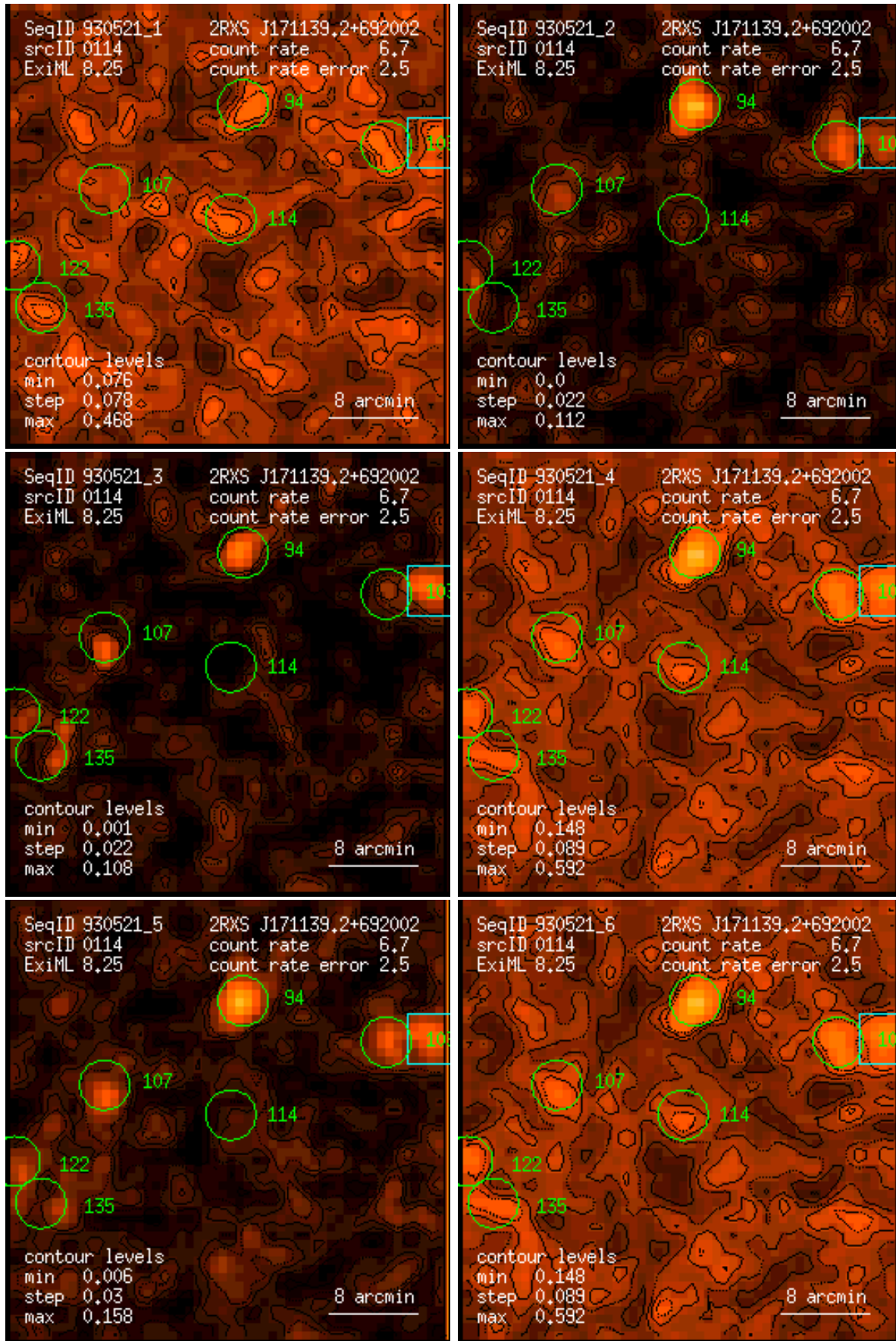
Figure 114: RASS 930521: detection 0114: band rate images, Gaussian filter: (1) PSPC channels 11 – 41, (2) 52 – 90, (3) 91 – 201, (4) 11 – 235, (5) 52 – 201, (6) 11 – 201. Broad band rates in counts/ks. Band rate contour levels in counts/ks/arcmin 2 .
