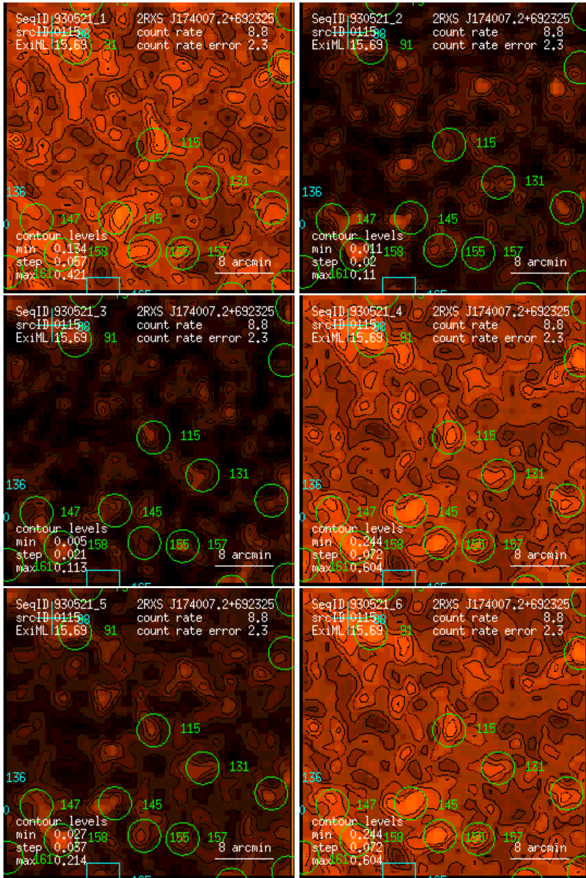
Figure 115: RASS 930521: detection 0115: band rate images, Gaussian filter: (1) PSPC channels 11 – 41, (2) 52 – 90, (3) 91 – 201, (4) 11 – 235, (5) 52 – 201, (6) 11 – 201. Broad band rates in counts/ks. Band rate contour levels in counts/ks/arcmin 2 .
