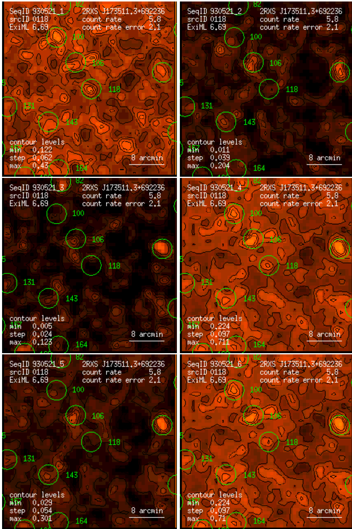
Figure 118: RASS 930521: detection 0118: band rate images, Gaussian filter: (1) PSPC channels 11 – 41, (2) 52 – 90, (3) 91 – 201, (4) 11 – 235, (5) 52 – 201, (6) 11 – 201. Broad band rates in counts/ks. Band rate contour levels in counts/ks/arcmin 2 .
