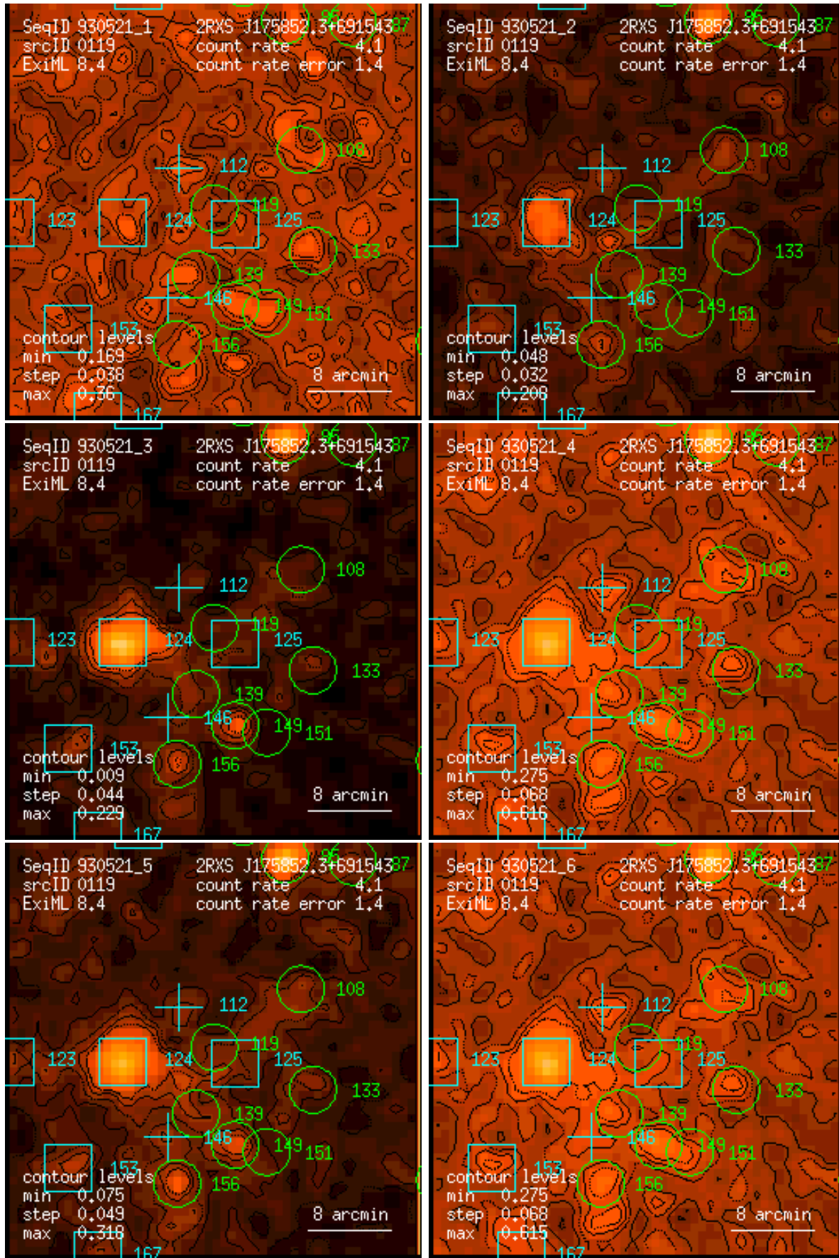
Figure 119: RASS 930521: detection 0119: band rate images, Gaussian filter: (1) PSPC channels 11 – 41, (2) 52 – 90, (3) 91 – 201, (4) 11 – 235, (5) 52 – 201, (6) 11 – 201. Broad band rates in counts/ks. Band rate contour levels in counts/ks/arcmin 2 .
