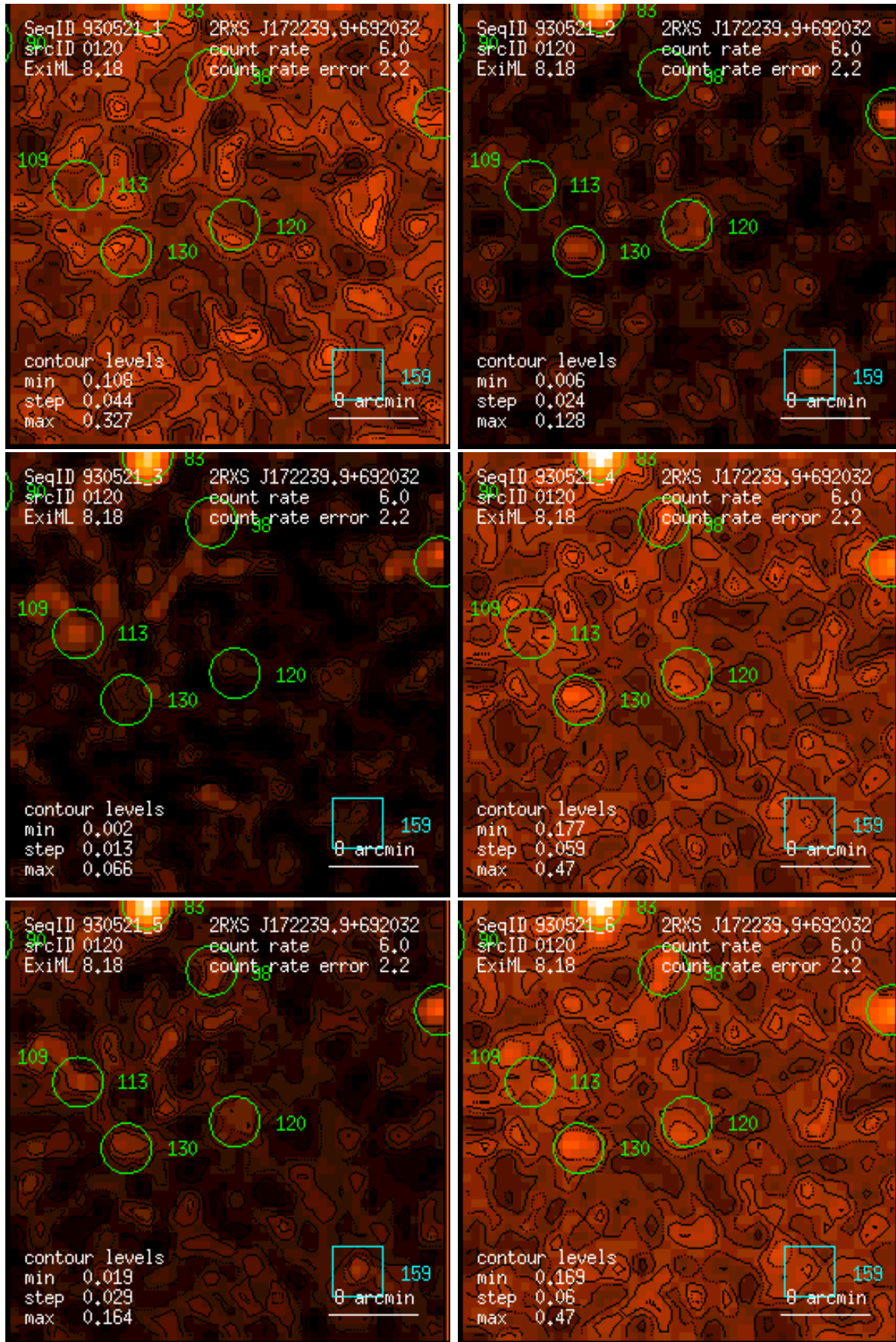
Figure 120: RASS 930521: detection 0120: band rate images, Gaussian filter: (1) PSPC channels 11 – 41, (2) 52 – 90, (3) 91 – 201, (4) 11 – 235, (5) 52 – 201, (6) 11 – 201. Broad band rates in counts/ks. Band rate contour levels in counts/ks/arcmin 2 .
