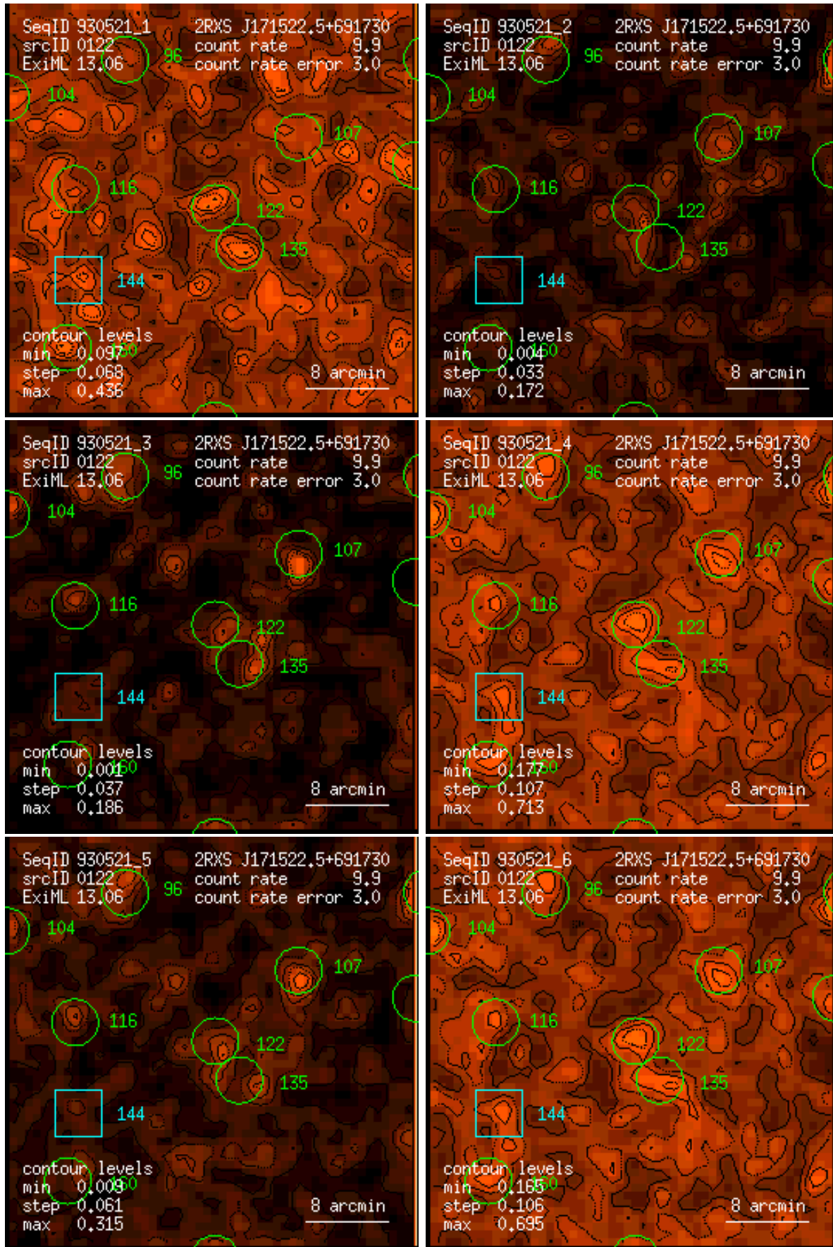
Figure 122: RASS 930521: detection 0122: band rate images, Gaussian filter: (1) PSPC channels 11 – 41, (2) 52 – 90, (3) 91 – 201, (4) 11 – 235, (5) 52 – 201, (6) 11 – 201. Broad band rates in counts/ks. Band rate contour levels in counts/ks/arcmin 2 .
