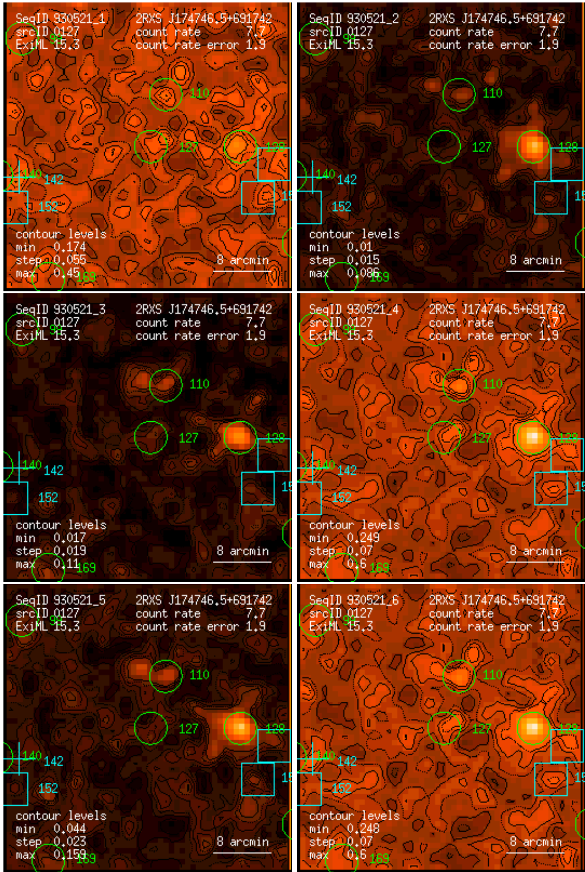
Figure 127: RASS 930521: detection 0127: band rate images, Gaussian filter: (1) PSPC channels 11 – 41, (2) 52 – 90, (3) 91 – 201, (4) 11 – 235, (5) 52 – 201, (6) 11 – 201. Broad band rates in counts/ks. Band rate contour levels in counts/ks/arcmin 2 .
