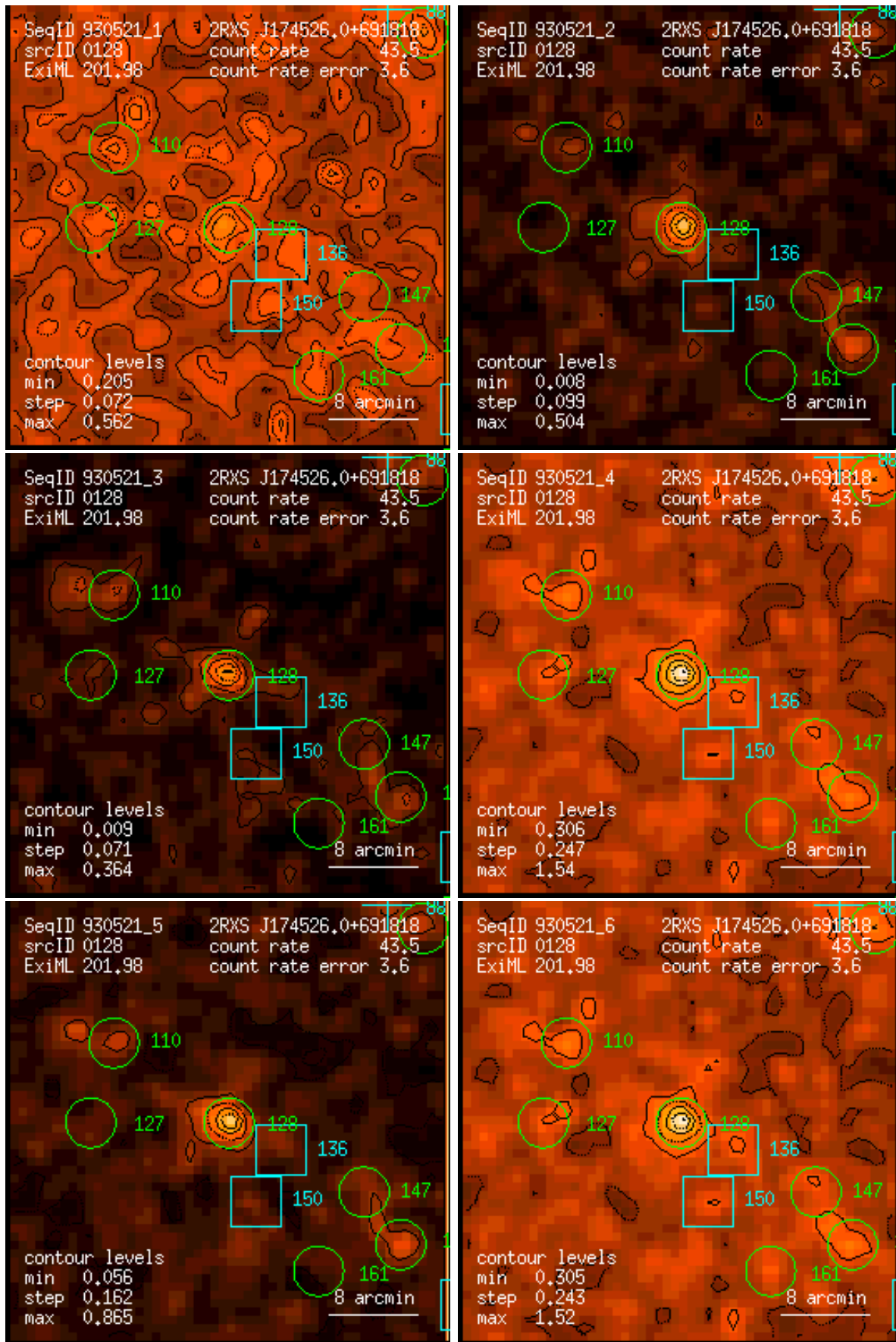
Figure 128: RASS 930521: detection 0128: band rate images, Gaussian filter: (1) PSPC channels 11 – 41, (2) 52 – 90, (3) 91 – 201, (4) 11 – 235, (5) 52 – 201, (6) 11 – 201. Broad band rates in counts/ks. Band rate contour levels in counts/ks/arcmin 2 .
