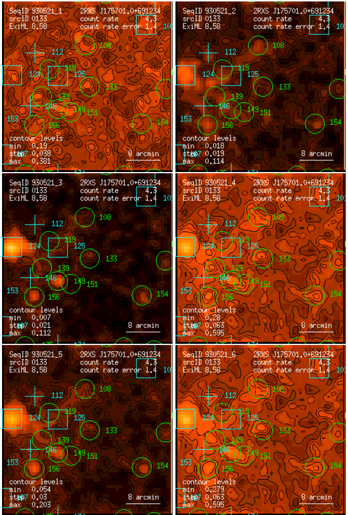
Figure 133: RASS 930521: detection 0133: band rate images, Gaussian filter: (1) PSPC channels 11 – 41, (2) 52 – 90, (3) 91 – 201, (4) 11 – 235, (5) 52 – 201, (6) 11 – 201. Broad band rates in counts/ks. Band rate contour levels in counts/ks/arcmin 2 .
