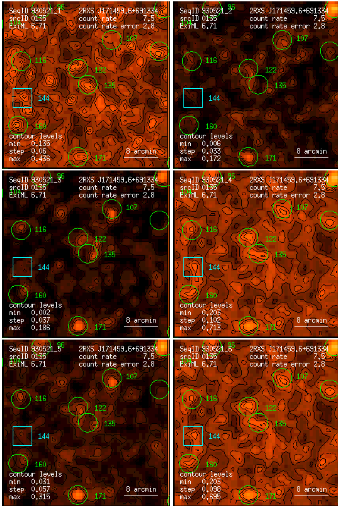
Figure 135: RASS 930521: detection 0135: band rate images, Gaussian filter: (1) PSPC channels 11 – 41, (2) 52 – 90, (3) 91 – 201, (4) 11 – 235, (5) 52 – 201, (6) 11 – 201. Broad band rates in counts/ks. Band rate contour levels in counts/ks/arcmin 2 .
