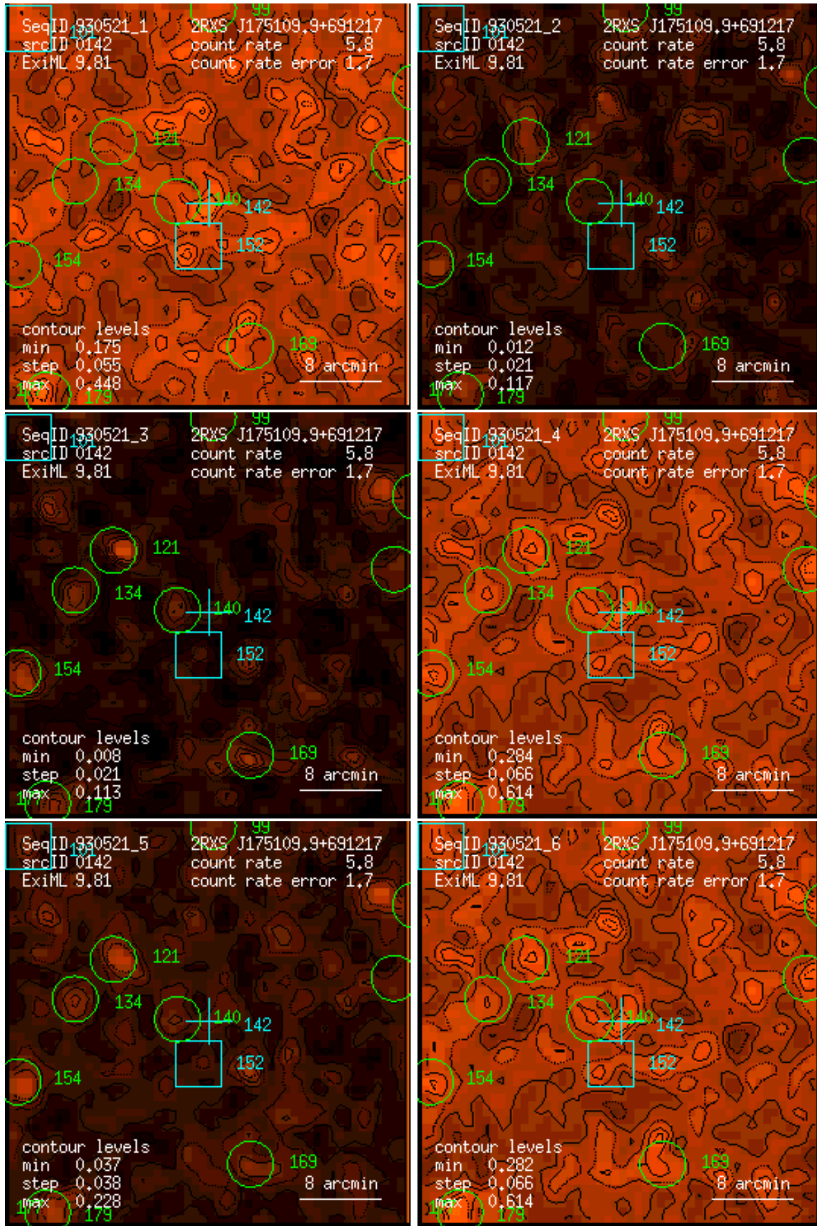
Figure 142: RASS 930521: detection 0142: band rate images, Gaussian filter: (1) PSPC channels 11 – 41, (2) 52 – 90, (3) 91 – 201, (4) 11 – 235, (5) 52 – 201, (6) 11 – 201. Broad band rates in counts/ks. Band rate contour levels in counts/ks/arcmin 2 .
