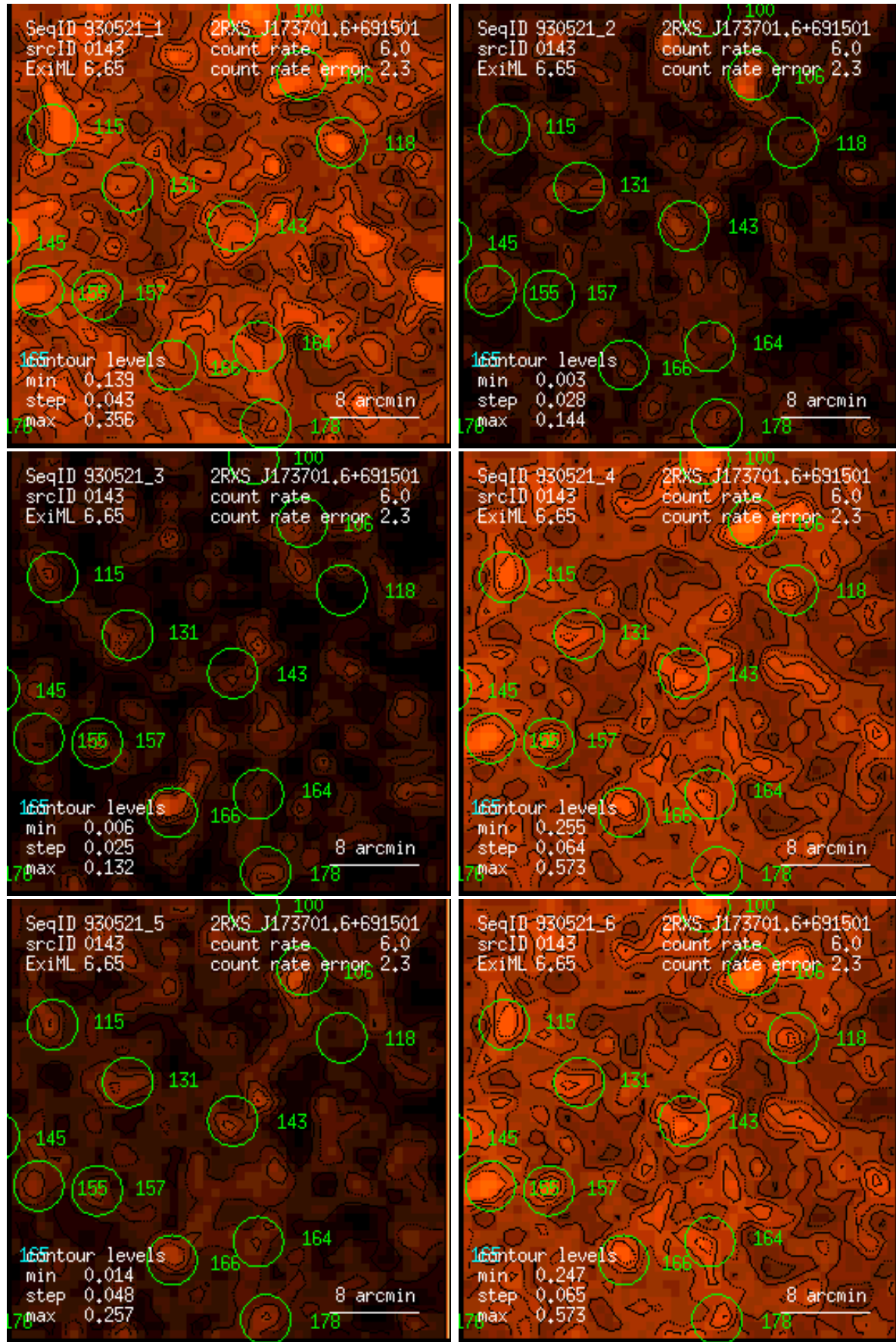
Figure 143: RASS 930521: detection 0143: band rate images, Gaussian filter: (1) PSPC channels 11 – 41, (2) 52 – 90, (3) 91 – 201, (4) 11 – 235, (5) 52 – 201, (6) 11 – 201. Broad band rates in counts/ks. Band rate contour levels in counts/ks/arcmin 2 .
