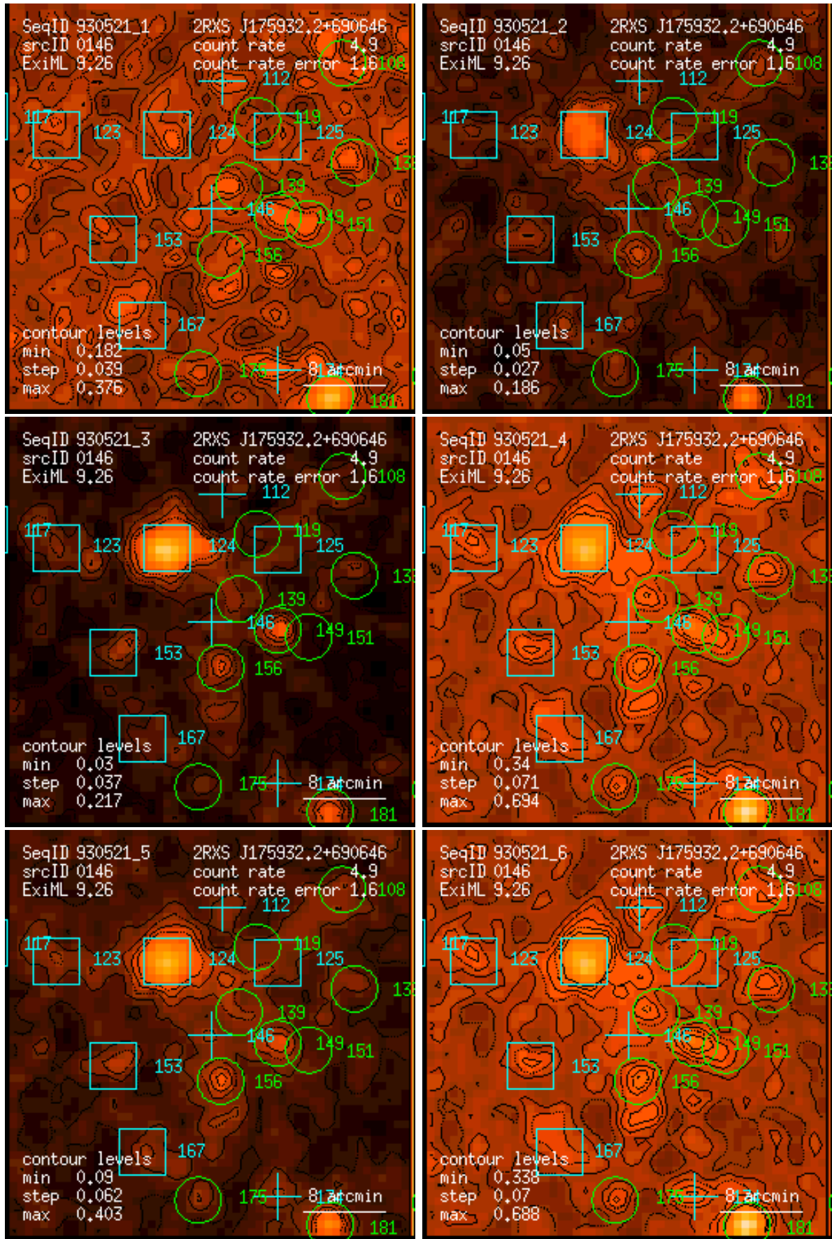
Figure 146: RASS 930521: detection 0146: band rate images, Gaussian filter: (1) PSPC channels 11 – 41, (2) 52 – 90, (3) 91 – 201, (4) 11 – 235, (5) 52 – 201, (6) 11 – 201. Broad band rates in counts/ks. Band rate contour levels in counts/ks/arcmin 2 .
