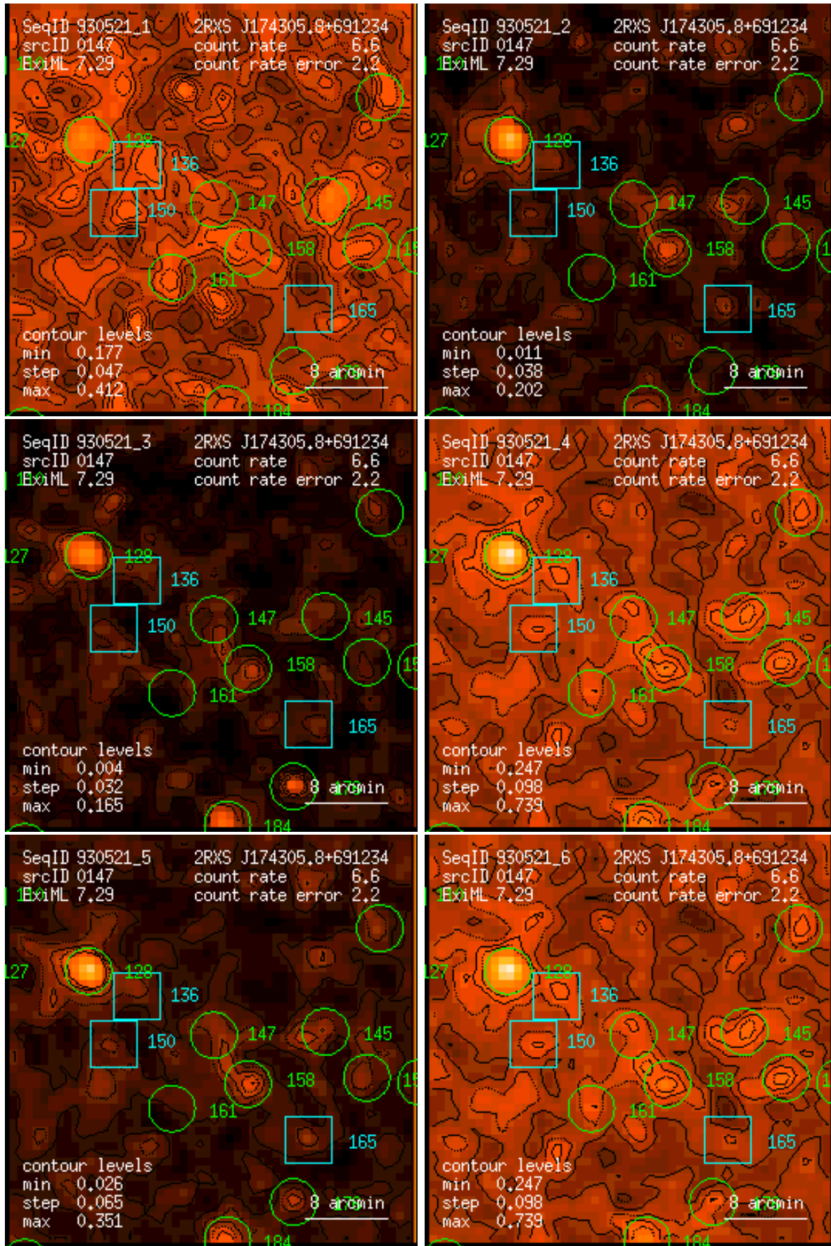
Figure 147: RASS 930521: detection 0147: band rate images, Gaussian filter: (1) PSPC channels 11 – 41, (2) 52 – 90, (3) 91 – 201, (4) 11 – 235, (5) 52 – 201, (6) 11 – 201. Broad band rates in counts/ks. Band rate contour levels in counts/ks/arcmin 2 .
