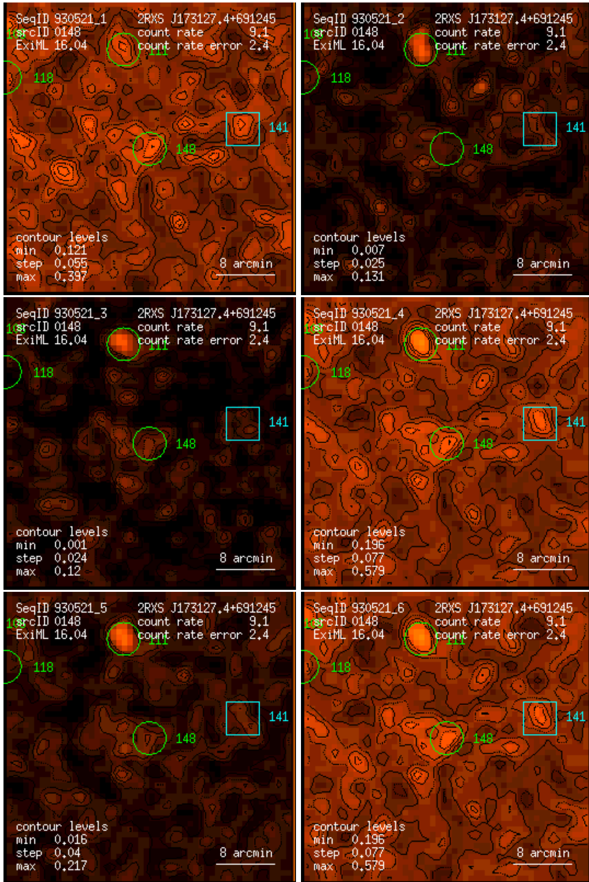
Figure 148: RASS 930521: detection 0148: band rate images, Gaussian filter: (1) PSPC channels 11 – 41, (2) 52 – 90, (3) 91 – 201, (4) 11 – 235, (5) 52 – 201, (6) 11 – 201. Broad band rates in counts/ks. Band rate contour levels in counts/ks/arcmin 2 .
