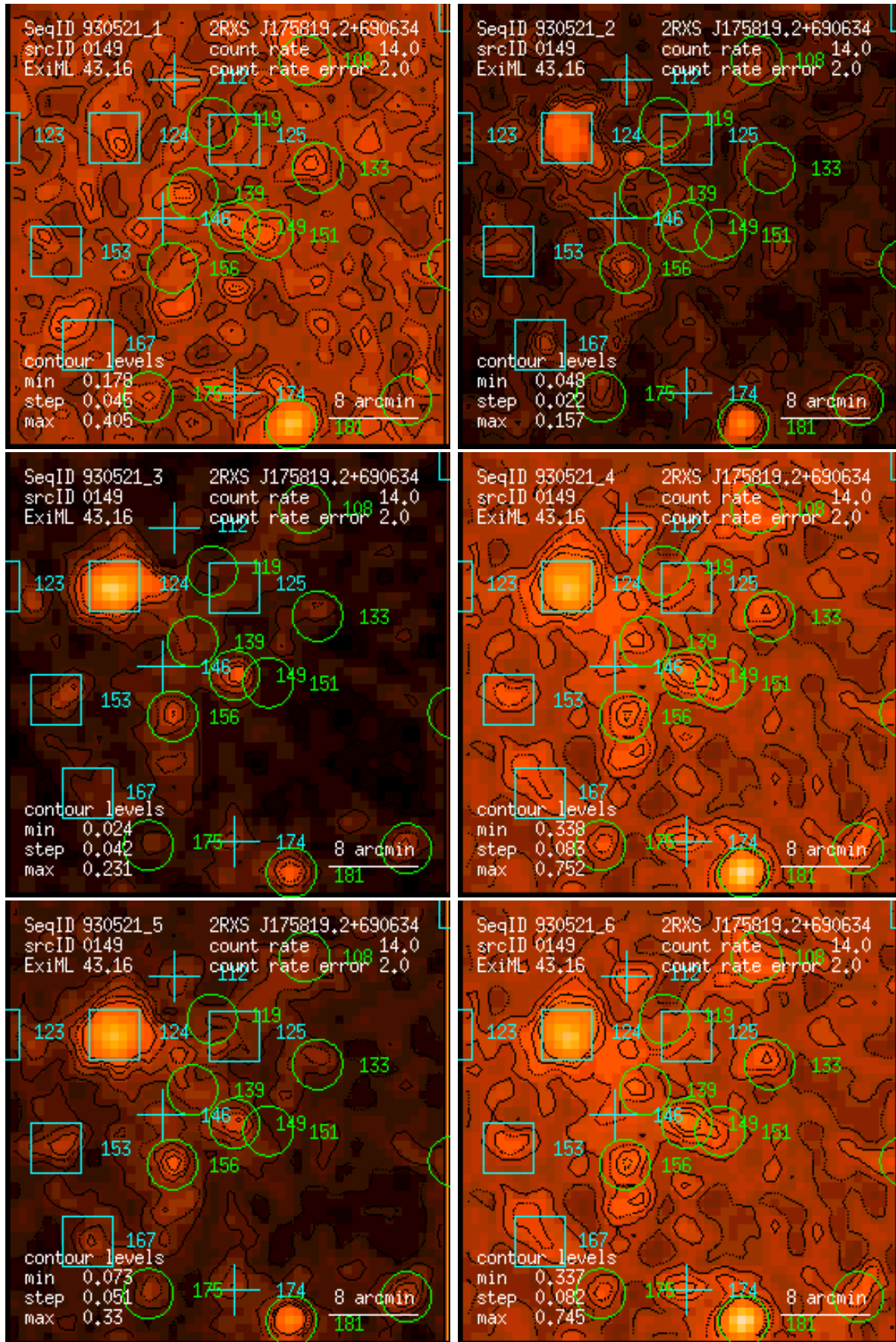
Figure 149: RASS 930521: detection 0149: band rate images, Gaussian filter: (1) PSPC channels 11 – 41, (2) 52 – 90, (3) 91 – 201, (4) 11 – 235, (5) 52 – 201, (6) 11 – 201. Broad band rates in counts/ks. Band rate contour levels in counts/ks/arcmin 2 .
