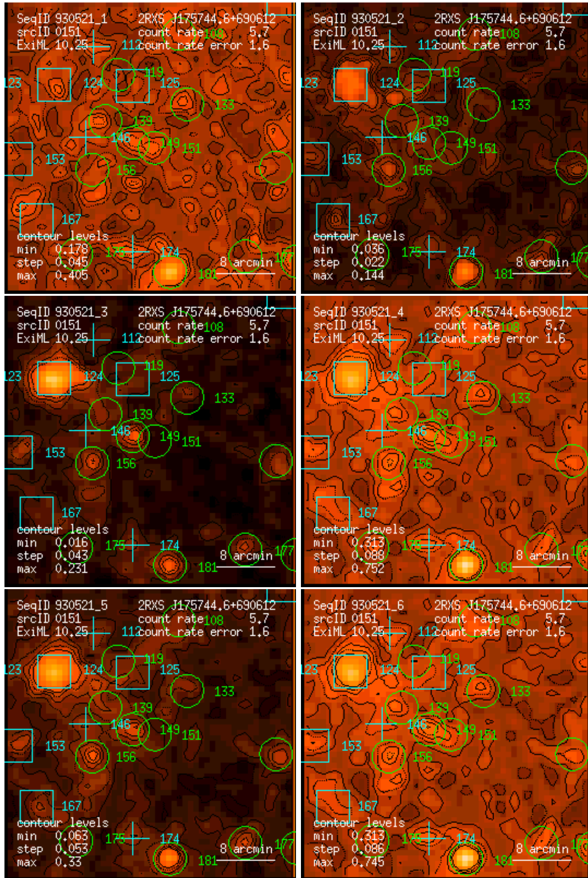
Figure 151: RASS 930521: detection 0151: band rate images, Gaussian filter: (1) PSPC channels 11 – 41, (2) 52 – 90, (3) 91 – 201, (4) 11 – 235, (5) 52 – 201, (6) 11 – 201. Broad band rates in counts/ks. Band rate contour levels in counts/ks/arcmin 2 .
