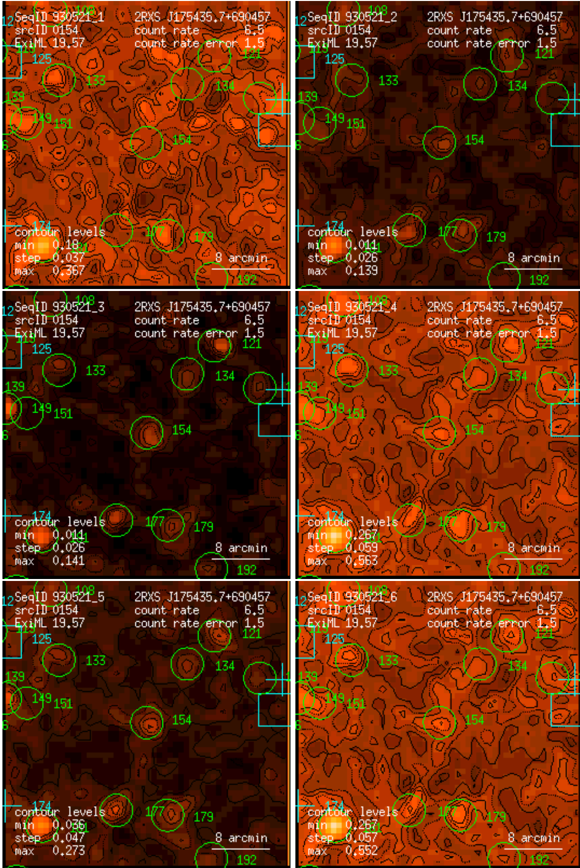
Figure 154: RASS 930521: detection 0154: band rate images, Gaussian filter: (1) PSPC channels 11 – 41, (2) 52 – 90, (3) 91 – 201, (4) 11 – 235, (5) 52 – 201, (6) 11 – 201. Broad band rates in counts/ks. Band rate contour levels in counts/ks/arcmin 2 .
