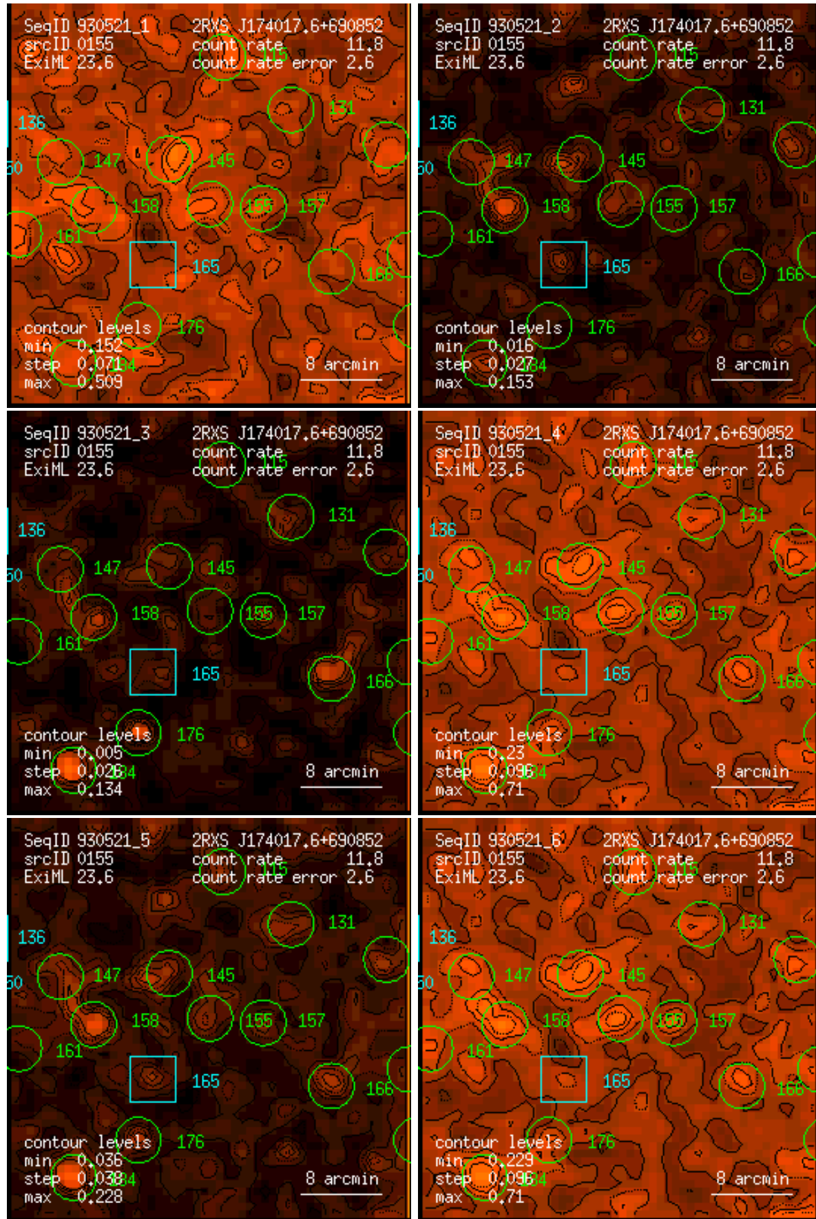
Figure 155: RASS 930521: detection 0155: band rate images, Gaussian filter: (1) PSPC channels 11 – 41, (2) 52 – 90, (3) 91 – 201, (4) 11 – 235, (5) 52 – 201, (6) 11 – 201. Broad band rates in counts/ks. Band rate contour levels in counts/ks/arcmin 2 .
