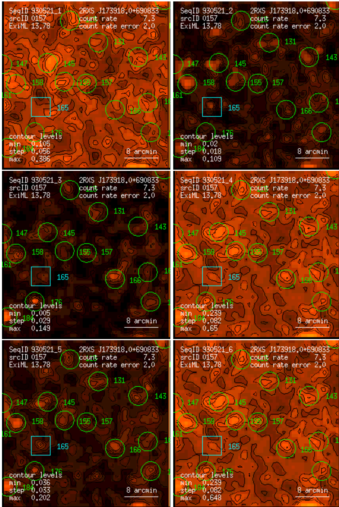
Figure 157: RASS 930521: detection 0157: band rate images, Gaussian filter: (1) PSPC channels 11 – 41, (2) 52 – 90, (3) 91 – 201, (4) 11 – 235, (5) 52 – 201, (6) 11 – 201. Broad band rates in counts/ks. Band rate contour levels in counts/ks/arcmin 2 .
