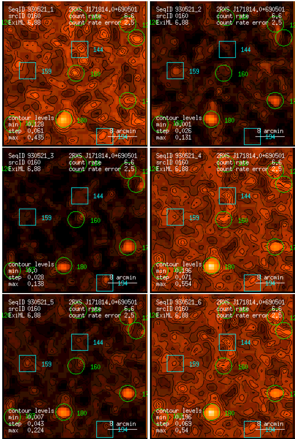
Figure 160: RASS 930521: detection 0160: band rate images, Gaussian filter: (1) PSPC channels 11 – 41, (2) 52 – 90, (3) 91 – 201, (4) 11 – 235, (5) 52 – 201, (6) 11 – 201. Broad band rates in counts/ks. Band rate contour levels in counts/ks/arcmin 2 .
