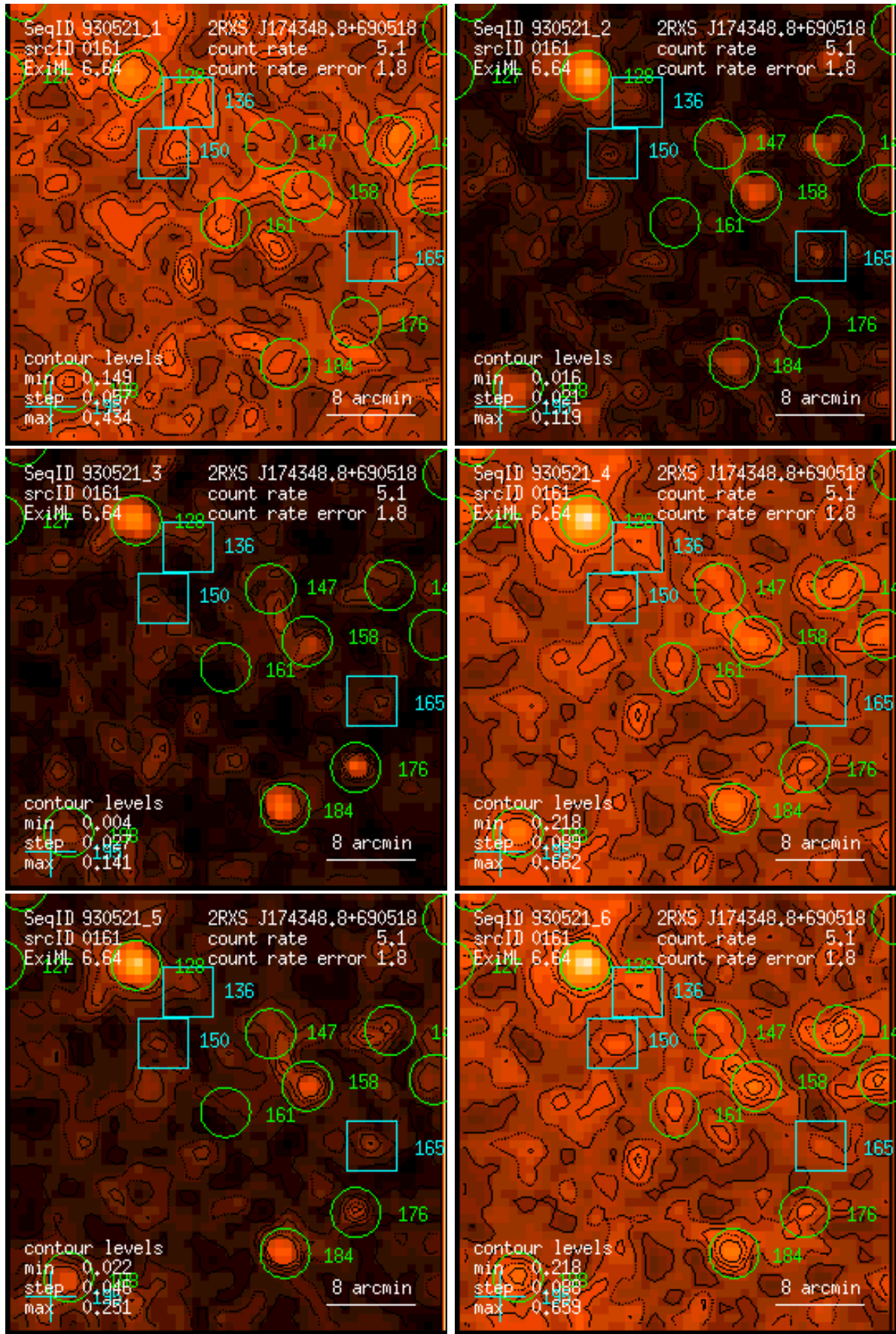
Figure 161: RASS 930521: detection 0161: band rate images, Gaussian filter: (1) PSPC channels 11 – 41, (2) 52 – 90, (3) 91 – 201, (4) 11 – 235, (5) 52 – 201, (6) 11 – 201. Broad band rates in counts/ks. Band rate contour levels in counts/ks/arcmin 2 .
