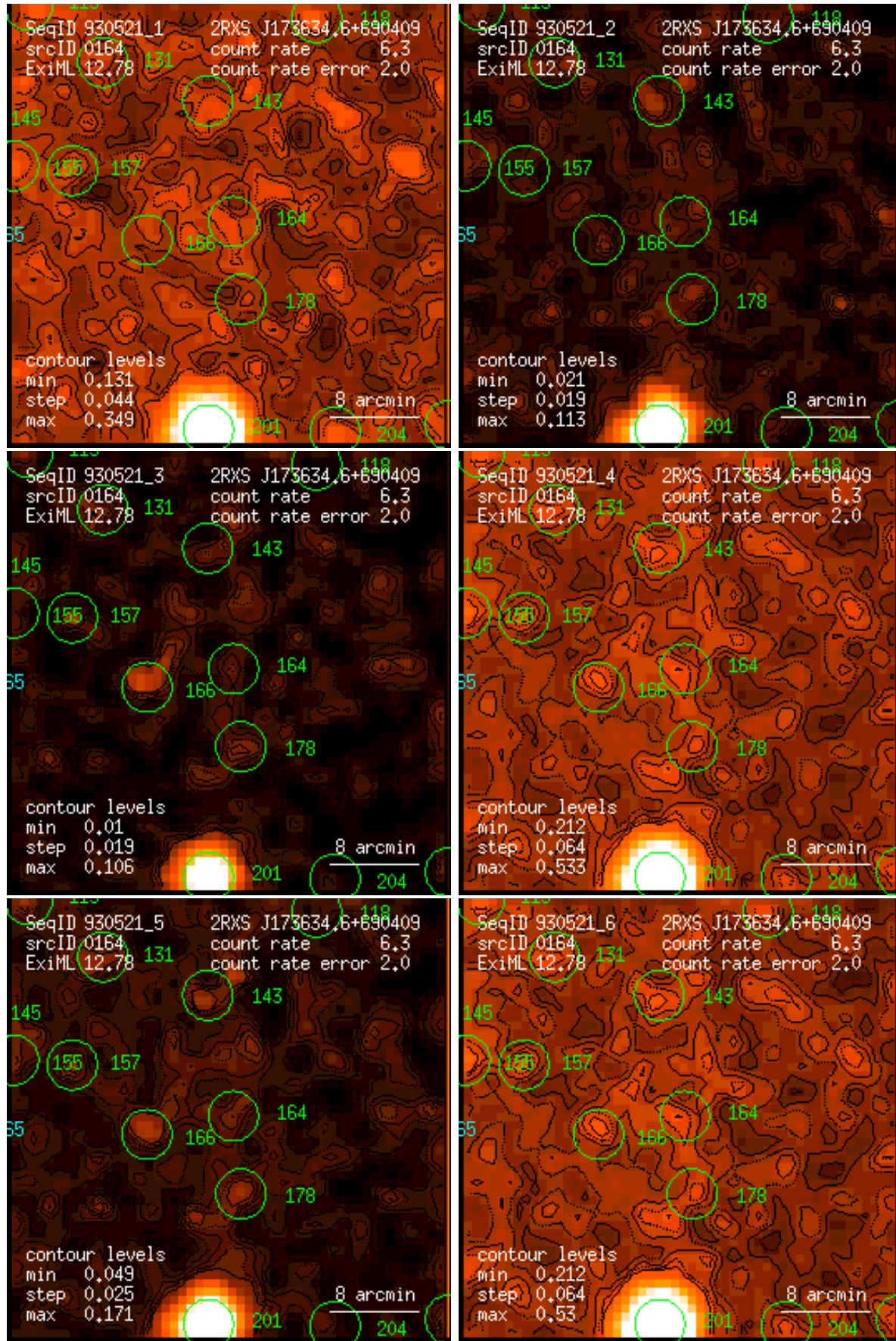
Figure 164: RASS 930521: detection 0164: band rate images, Gaussian filter: (1) PSPC channels 11 – 41, (2) 52 – 90, (3) 91 – 201, (4) 11 – 235, (5) 52 – 201, (6) 11 – 201. Broad band rates in counts/ks. Band rate contour levels in counts/ks/arcmin 2 .
