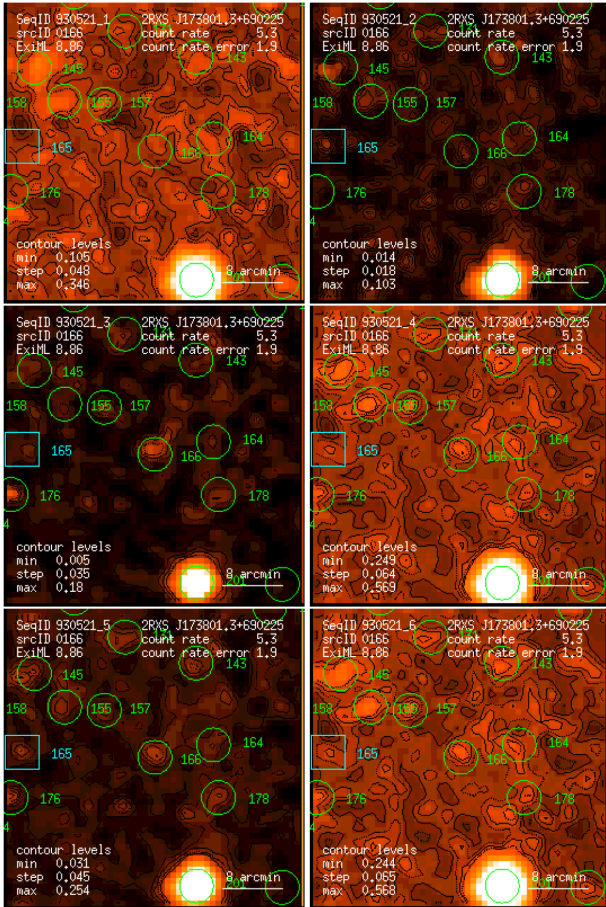
Figure 166: RASS 930521: detection 0166: band rate images, Gaussian filter: (1) PSPC channels 11 – 41, (2) 52 – 90, (3) 91 – 201, (4) 11 – 235, (5) 52 – 201, (6) 11 – 201. Broad band rates in counts/ks. Band rate contour levels in counts/ks/arcmin 2 .
