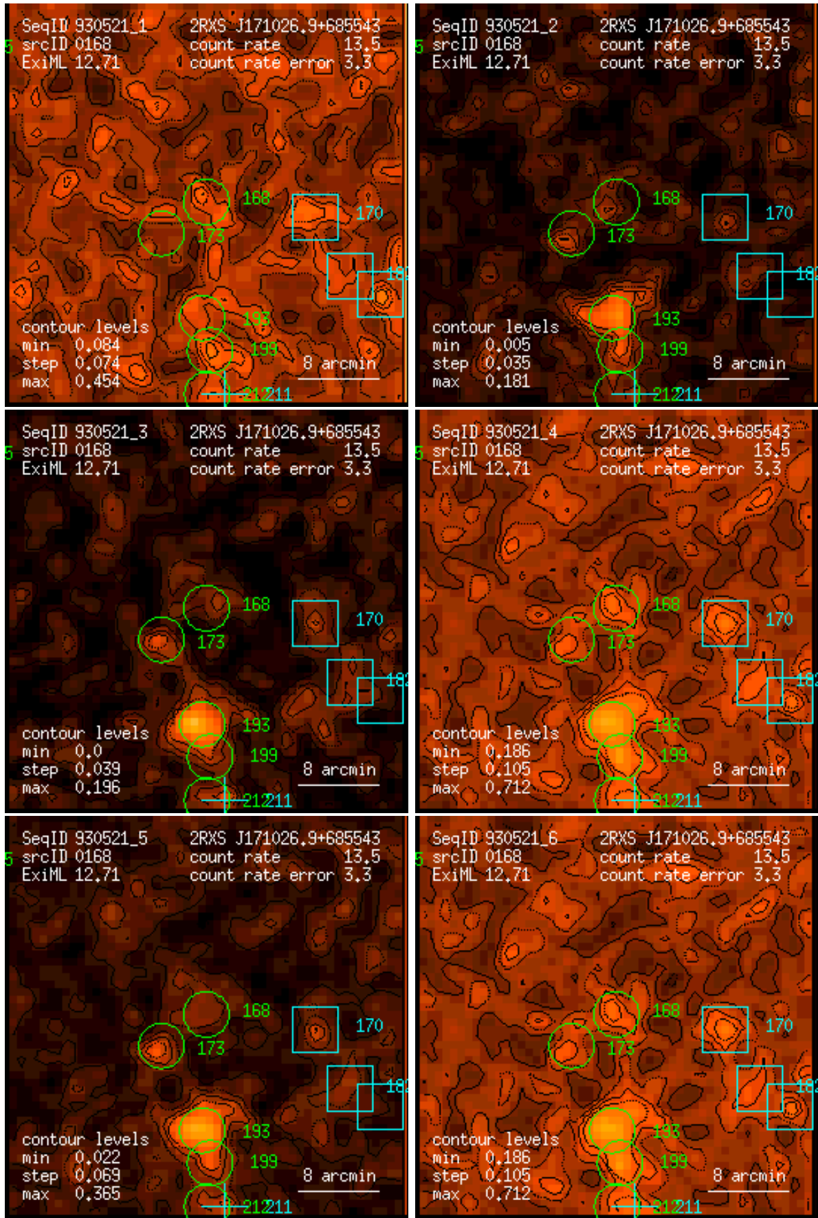
Figure 168: RASS 930521: detection 0168: band rate images, Gaussian filter: (1) PSPC channels 11 – 41, (2) 52 – 90, (3) 91 – 201, (4) 11 – 235, (5) 52 – 201, (6) 11 – 201. Broad band rates in counts/ks. Band rate contour levels in counts/ks/arcmin 2 .
