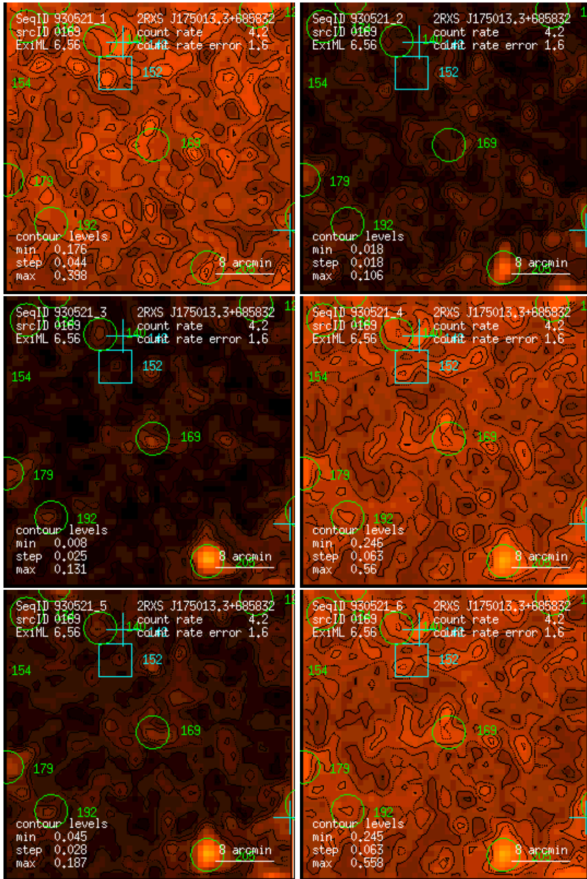
Figure 169: RASS 930521: detection 0169: band rate images, Gaussian filter: (1) PSPC channels 11 – 41, (2) 52 – 90, (3) 91 – 201, (4) 11 – 235, (5) 52 – 201, (6) 11 – 201. Broad band rates in counts/ks. Band rate contour levels in counts/ks/arcmin 2 .
