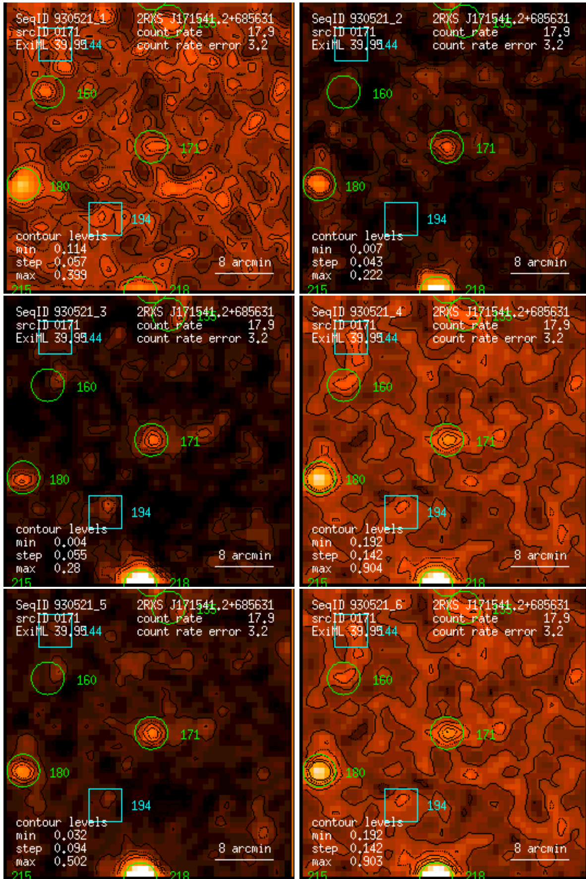
Figure 171: RASS 930521: detection 0171: band rate images, Gaussian filter: (1) PSPC channels 11 – 41, (2) 52 – 90, (3) 91 – 201, (4) 11 – 235, (5) 52 – 201, (6) 11 – 201. Broad band rates in counts/ks. Band rate contour levels in counts/ks/arcmin 2 .
