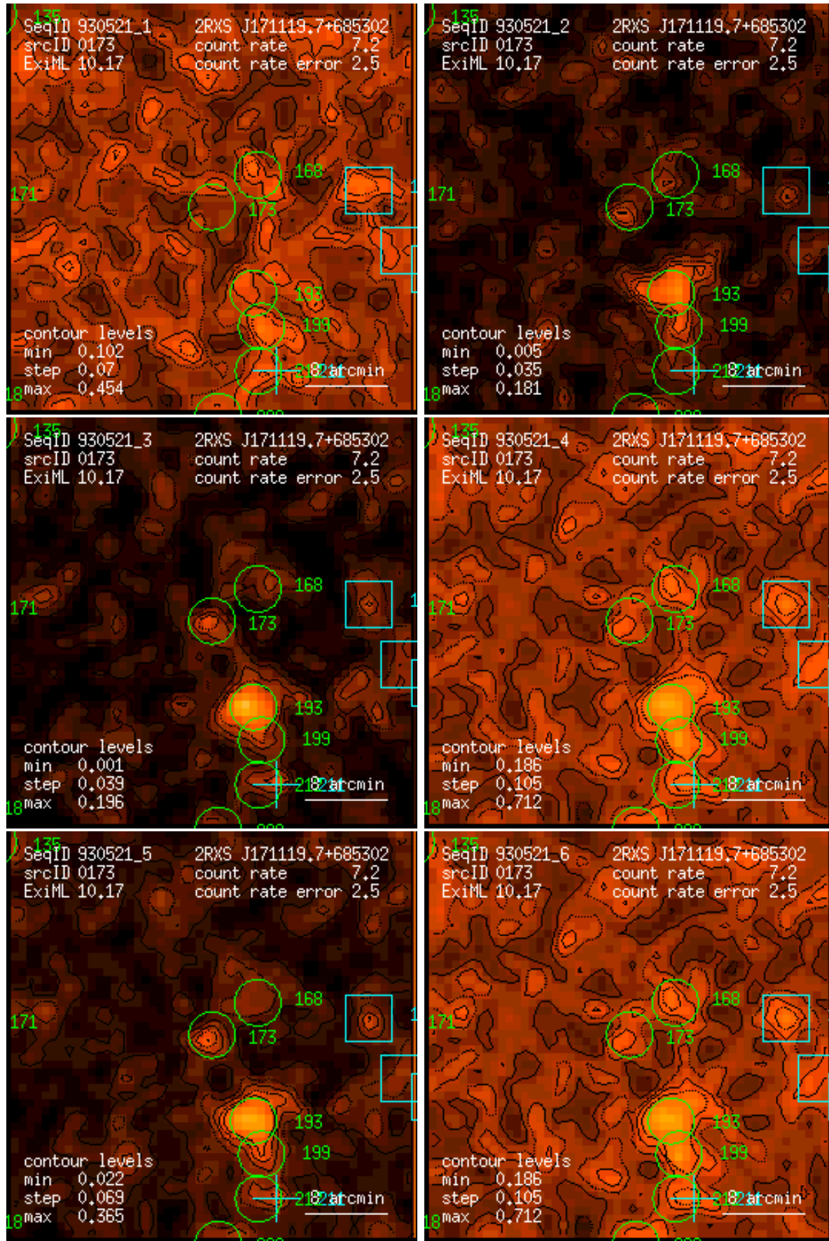
Figure 173: RASS 930521: detection 0173: band rate images, Gaussian filter: (1) PSPC channels 11 – 41, (2) 52 – 90, (3) 91 – 201, (4) 11 – 235, (5) 52 – 201, (6) 11 – 201. Broad band rates in counts/ks. Band rate contour levels in counts/ks/arcmin 2 .
