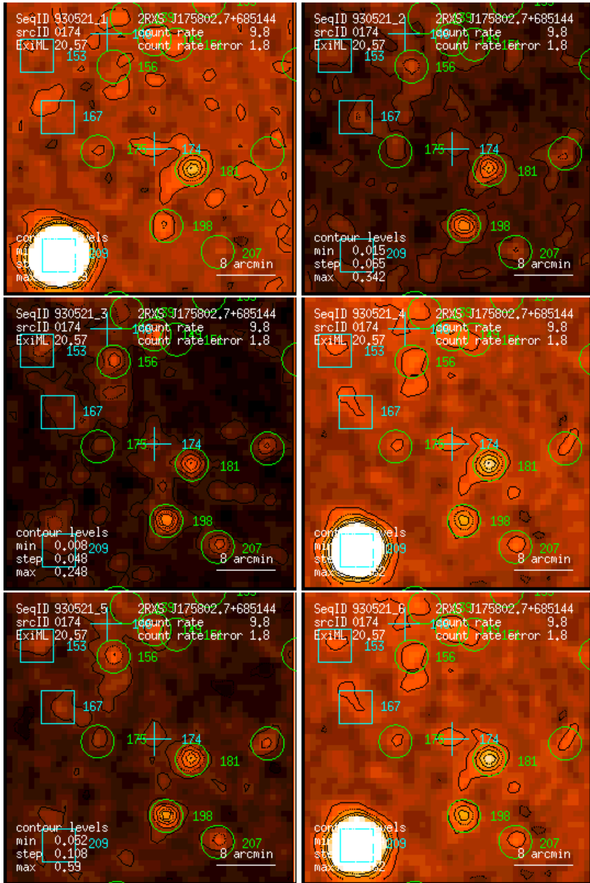
Figure 174: RASS 930521: detection 0174: band rate images, Gaussian filter: (1) PSPC channels 11 – 41, (2) 52 – 90, (3) 91 – 201, (4) 11 – 235, (5) 52 – 201, (6) 11 – 201. Broad band rates in counts/ks. Band rate contour levels in counts/ks/arcmin 2 .
