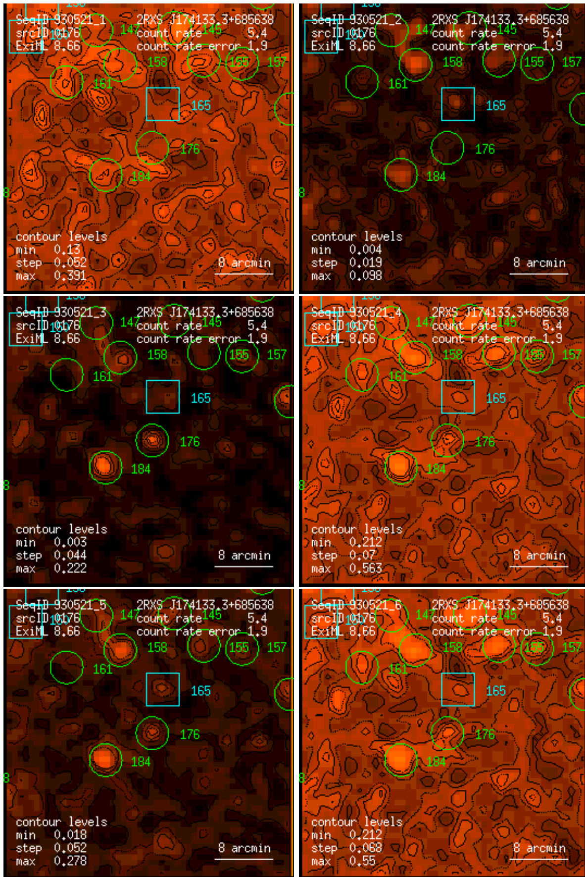
Figure 176: RASS 930521: detection 0176: band rate images, Gaussian filter: (1) PSPC channels 11 – 41, (2) 52 – 90, (3) 91 – 201, (4) 11 – 235, (5) 52 – 201, (6) 11 – 201. Broad band rates in counts/ks. Band rate contour levels in counts/ks/arcmin 2 .
