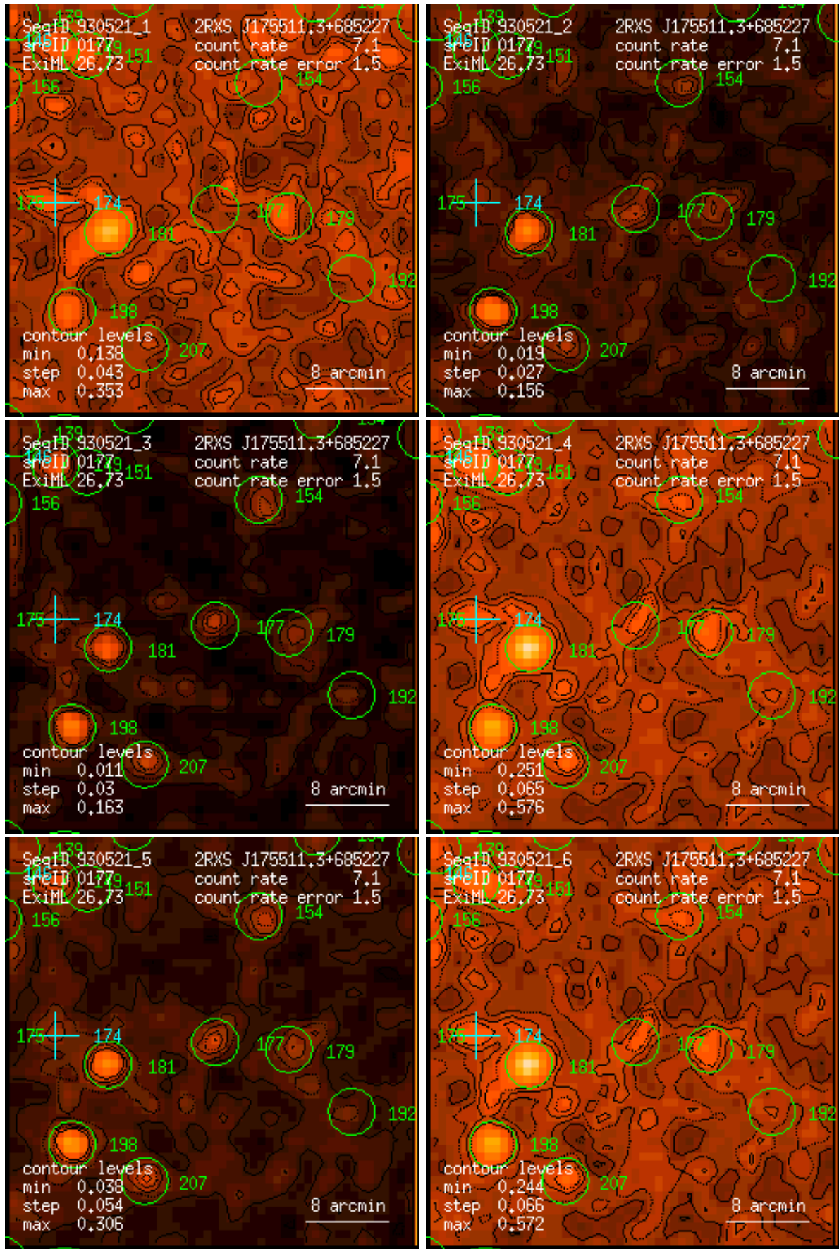
Figure 177: RASS 930521: detection 0177: band rate images, Gaussian filter: (1) PSPC channels 11 – 41, (2) 52 – 90, (3) 91 – 201, (4) 11 – 235, (5) 52 – 201, (6) 11 – 201. Broad band rates in counts/ks. Band rate contour levels in counts/ks/arcmin 2 .
