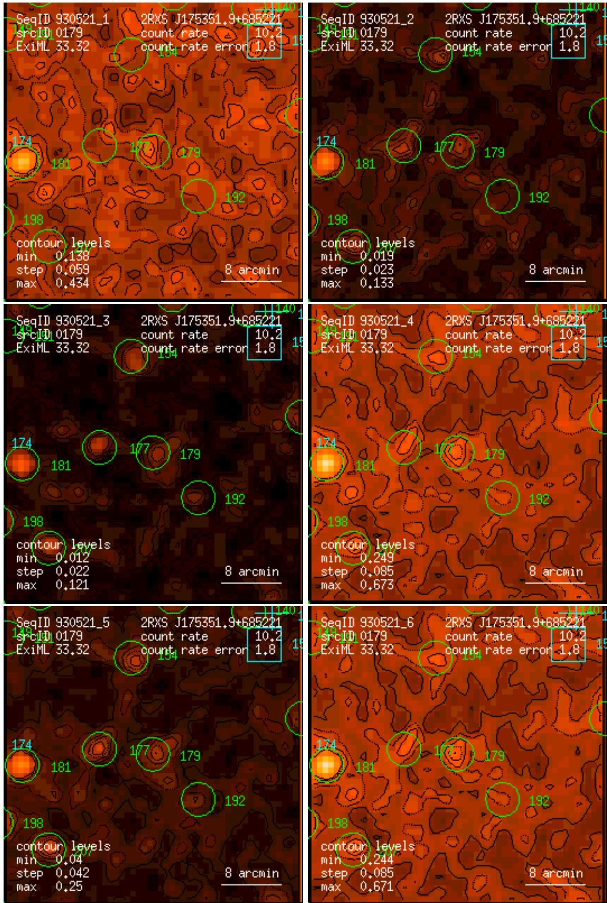
Figure 179: RASS 930521: detection 0179: band rate images, Gaussian filter: (1) PSPC channels 11 – 41, (2) 52 – 90, (3) 91 – 201, (4) 11 – 235, (5) 52 – 201, (6) 11 – 201. Broad band rates in counts/ks. Band rate contour levels in counts/ks/arcmin 2 .
