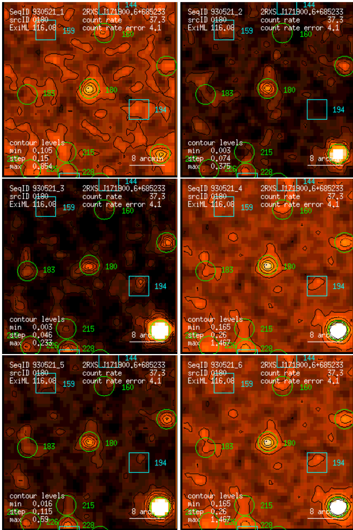
Figure 180: RASS 930521: detection 0180: band rate images, Gaussian filter: (1) PSPC channels 11 – 41, (2) 52 – 90, (3) 91 – 201, (4) 11 – 235, (5) 52 – 201, (6) 11 – 201. Broad band rates in counts/ks. Band rate contour levels in counts/ks/arcmin 2 .
