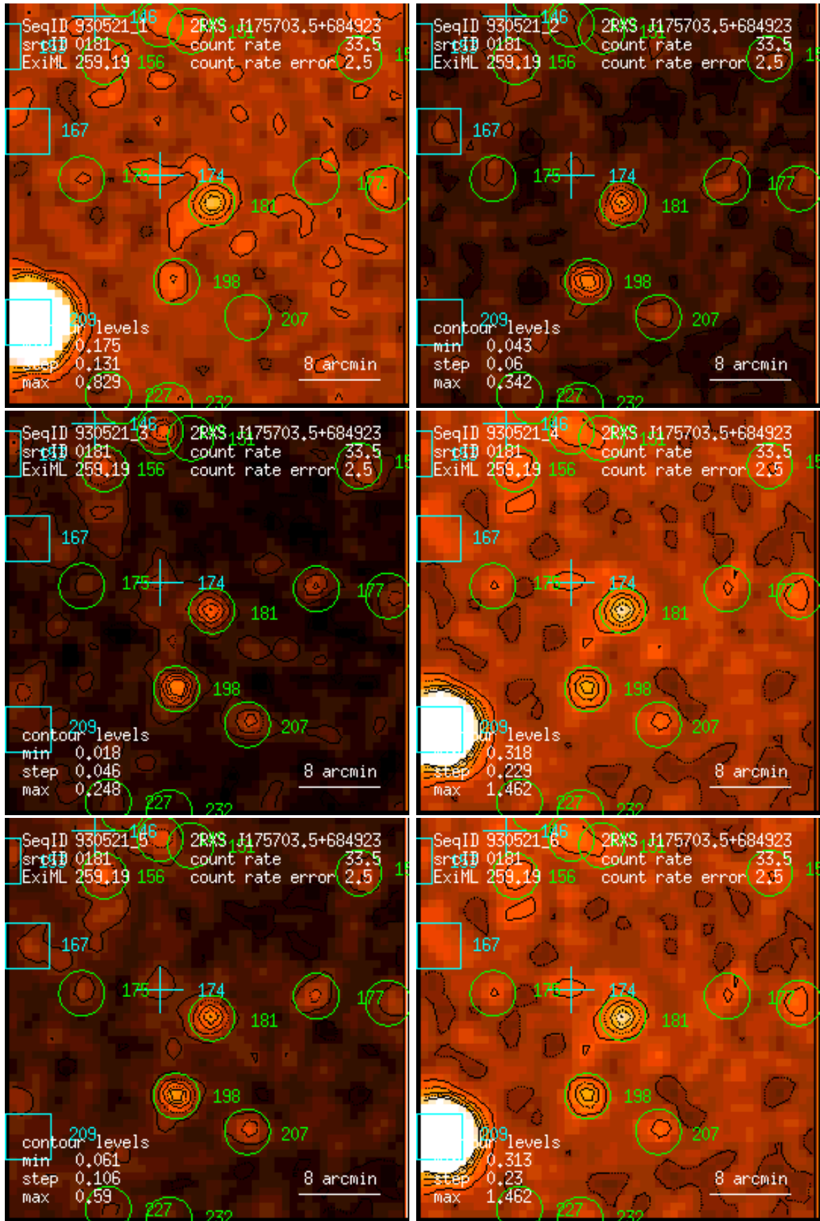
Figure 181: RASS 930521: detection 0181: band rate images, Gaussian filter: (1) PSPC channels 11 – 41, (2) 52 – 90, (3) 91 – 201, (4) 11 – 235, (5) 52 – 201, (6) 11 – 201. Broad band rates in counts/ks. Band rate contour levels in counts/ks/arcmin 2 .
