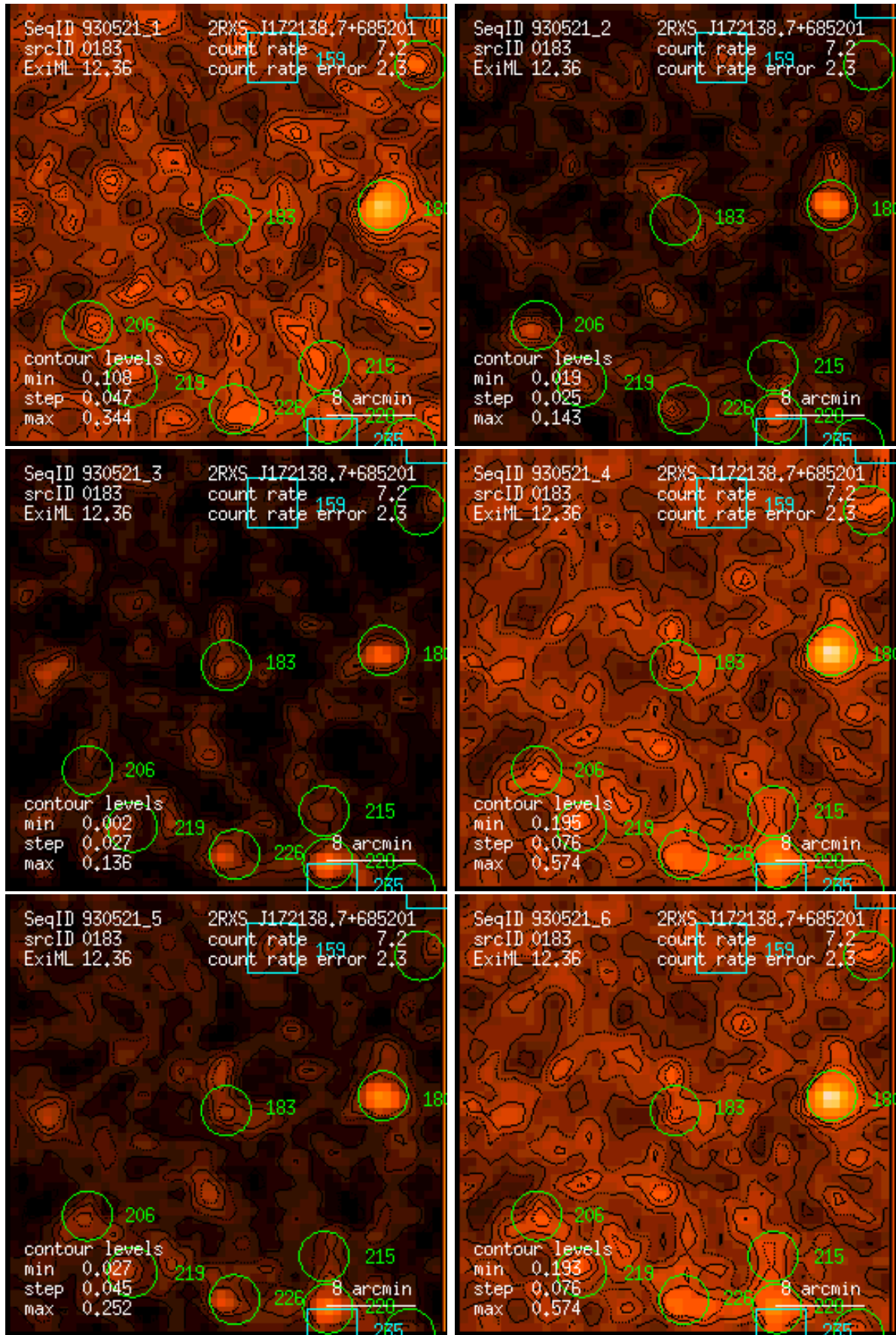
Figure 183: RASS 930521: detection 0183: band rate images, Gaussian filter: (1) PSPC channels 11 – 41, (2) 52 – 90, (3) 91 – 201, (4) 11 – 235, (5) 52 – 201, (6) 11 – 201. Broad band rates in counts/ks. Band rate contour levels in counts/ks/arcmin 2 .
