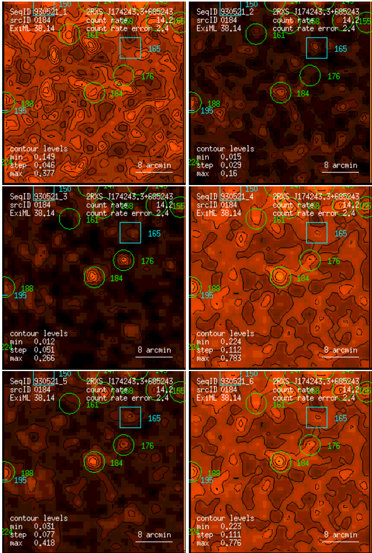
Figure 184: RASS 930521: detection 0184: band rate images, Gaussian filter: (1) PSPC channels 11 – 41, (2) 52 – 90, (3) 91 – 201, (4) 11 – 235, (5) 52 – 201, (6) 11 – 201. Broad band rates in counts/ks. Band rate contour levels in counts/ks/arcmin 2 .
