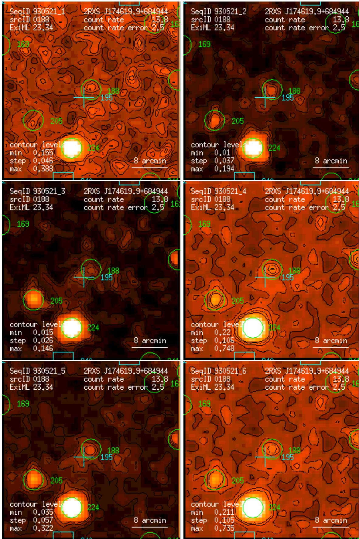
Figure 188: RASS 930521: detection 0188: band rate images, Gaussian filter: (1) PSPC channels 11 – 41, (2) 52 – 90, (3) 91 – 201, (4) 11 – 235, (5) 52 – 201, (6) 11 – 201. Broad band rates in counts/ks. Band rate contour levels in counts/ks/arcmin 2 .
