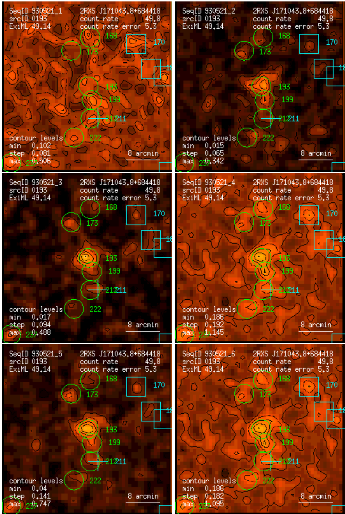
Figure 193: RASS 930521: detection 0193: band rate images, Gaussian filter: (1) PSPC channels 11 – 41, (2) 52 – 90, (3) 91 – 201, (4) 11 – 235, (5) 52 – 201, (6) 11 – 201. Broad band rates in counts/ks. Band rate contour levels in counts/ks/arcmin 2 .
