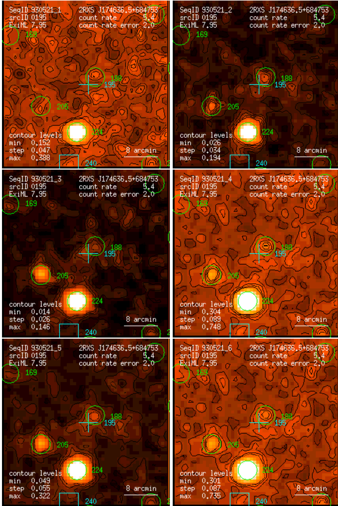
Figure 195: RASS 930521: detection 0195: band rate images, Gaussian filter: (1) PSPC channels 11 – 41, (2) 52 – 90, (3) 91 – 201, (4) 11 – 235, (5) 52 – 201, (6) 11 – 201. Broad band rates in counts/ks. Band rate contour levels in counts/ks/arcmin 2 .
