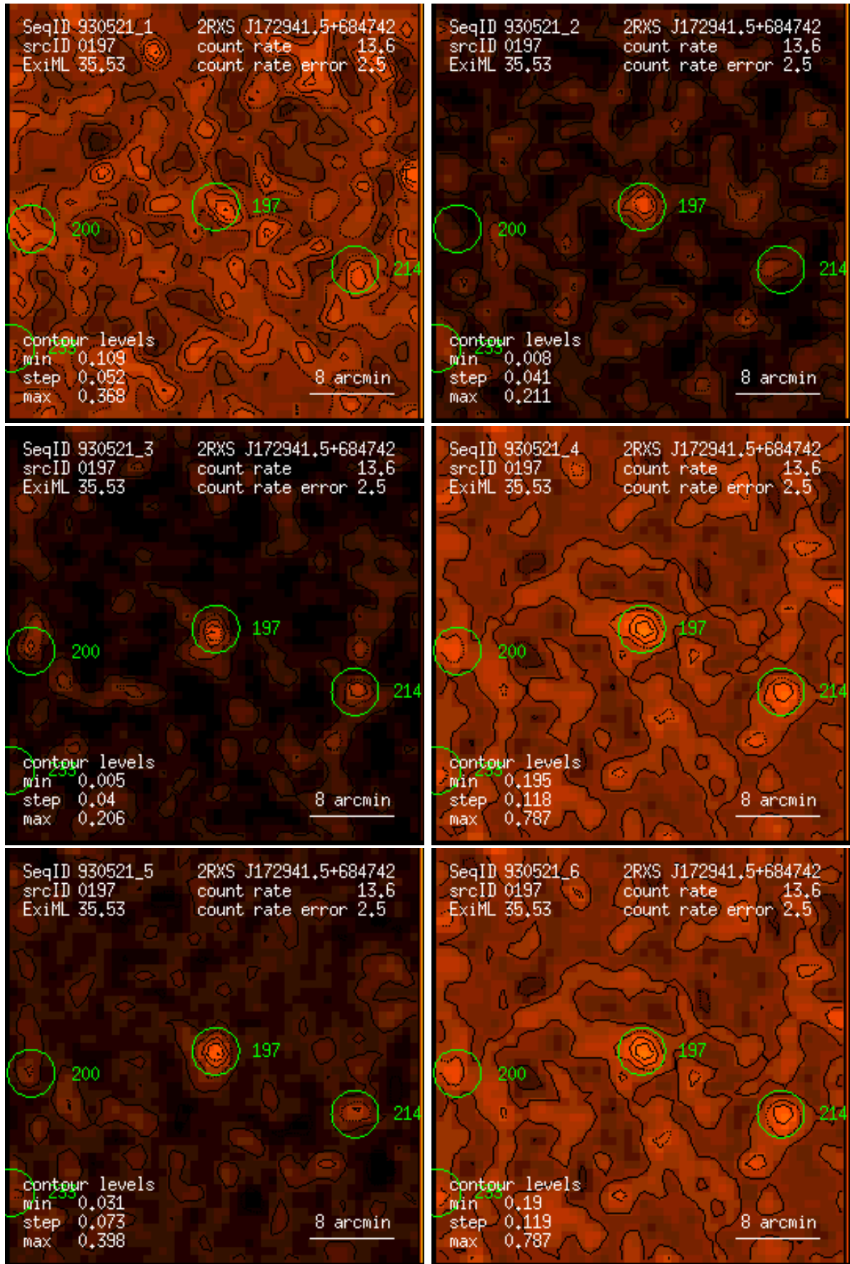
Figure 197: RASS 930521: detection 0197: band rate images, Gaussian filter: (1) PSPC channels 11 – 41, (2) 52 – 90, (3) 91 – 201, (4) 11 – 235, (5) 52 – 201, (6) 11 – 201. Broad band rates in counts/ks. Band rate contour levels in counts/ks/arcmin 2 .
