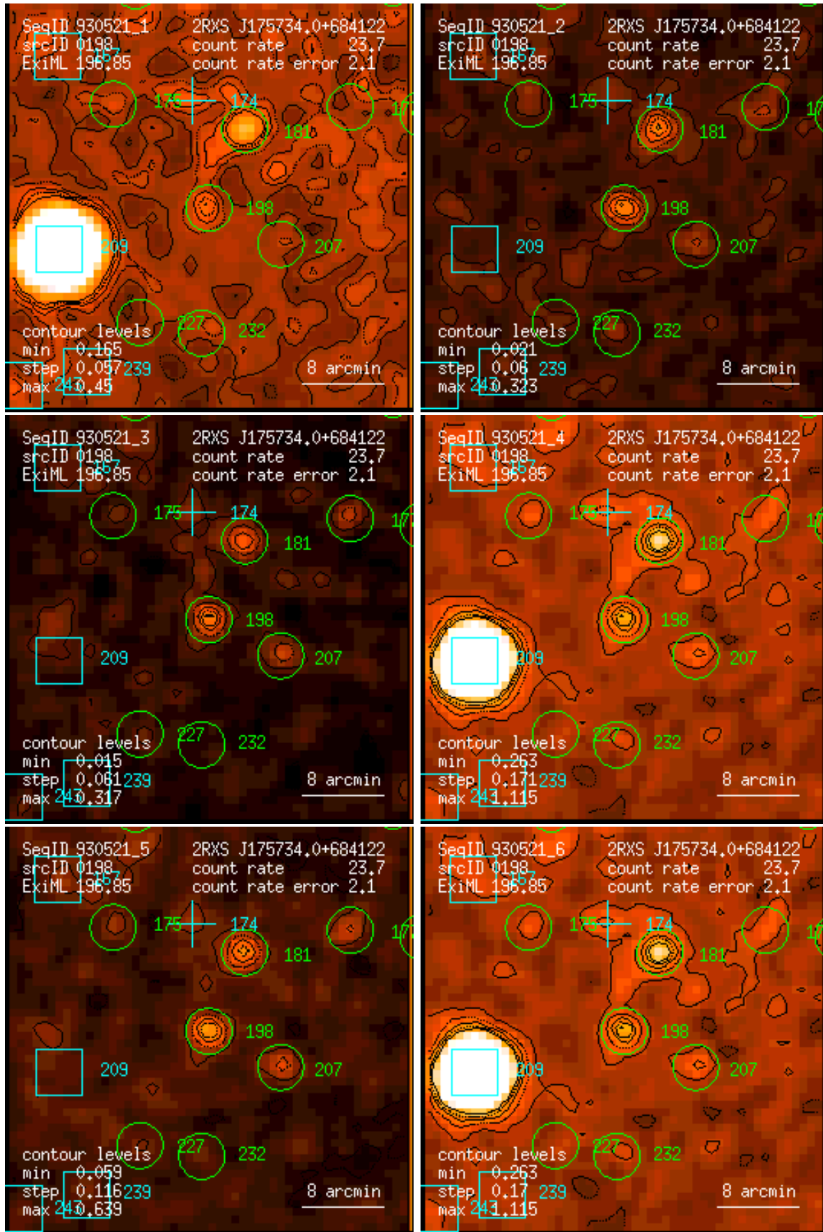
Figure 198: RASS 930521: detection 0198: band rate images, Gaussian filter: (1) PSPC channels 11 – 41, (2) 52 – 90, (3) 91 – 201, (4) 11 – 235, (5) 52 – 201, (6) 11 – 201. Broad band rates in counts/ks. Band rate contour levels in counts/ks/arcmin 2 .
