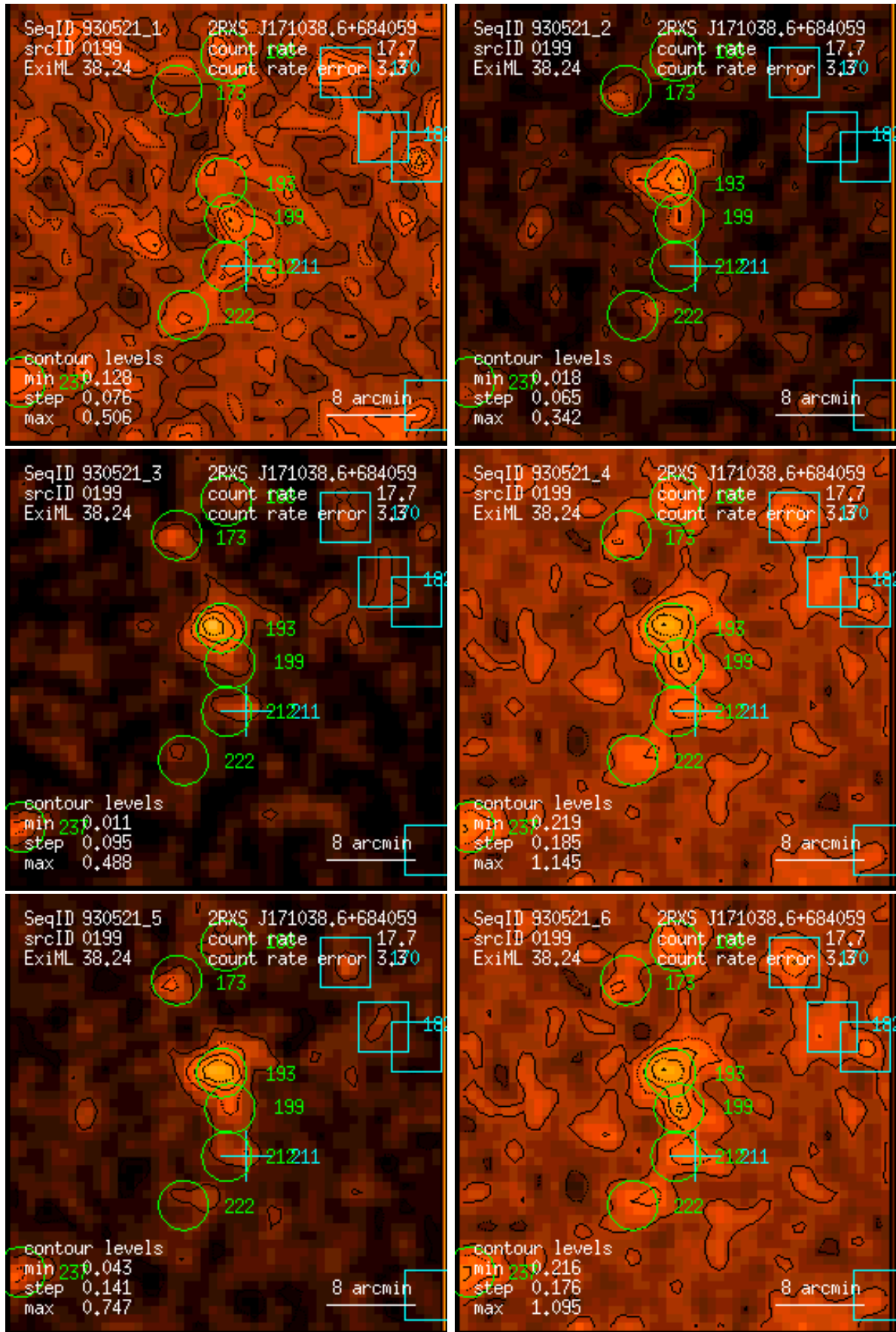
Figure 199: RASS 930521: detection 0199: band rate images, Gaussian filter: (1) PSPC channels 11 – 41, (2) 52 – 90, (3) 91 – 201, (4) 11 – 235, (5) 52 – 201, (6) 11 – 201. Broad band rates in counts/ks. Band rate contour levels in counts/ks/arcmin 2 .
