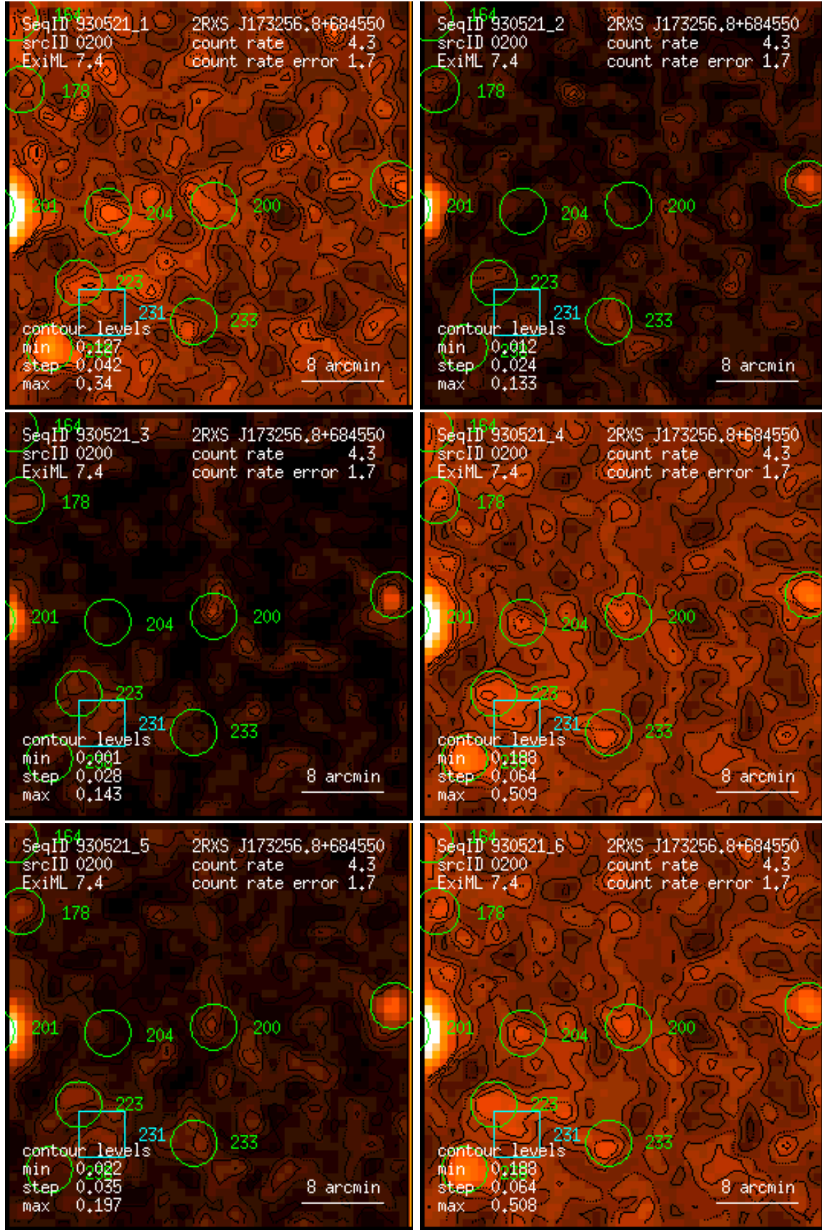
Figure 200: RASS 930521: detection 0200: band rate images, Gaussian filter: (1) PSPC channels 11 – 41, (2) 52 – 90, (3) 91 – 201, (4) 11 – 235, (5) 52 – 201, (6) 11 – 201. Broad band rates in counts/ks. Band rate contour levels in counts/ks/arcmin 2 .
