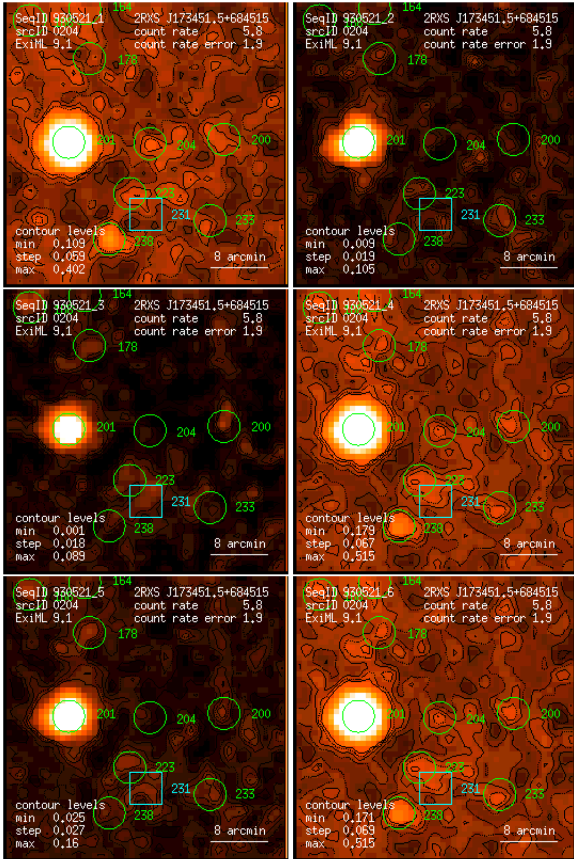
Figure 204: RASS 930521: detection 0204: band rate images, Gaussian filter: (1) PSPC channels 11 – 41, (2) 52 – 90, (3) 91 – 201, (4) 11 – 235, (5) 52 – 201, (6) 11 – 201. Broad band rates in counts/ks. Band rate contour levels in counts/ks/arcmin 2 .
