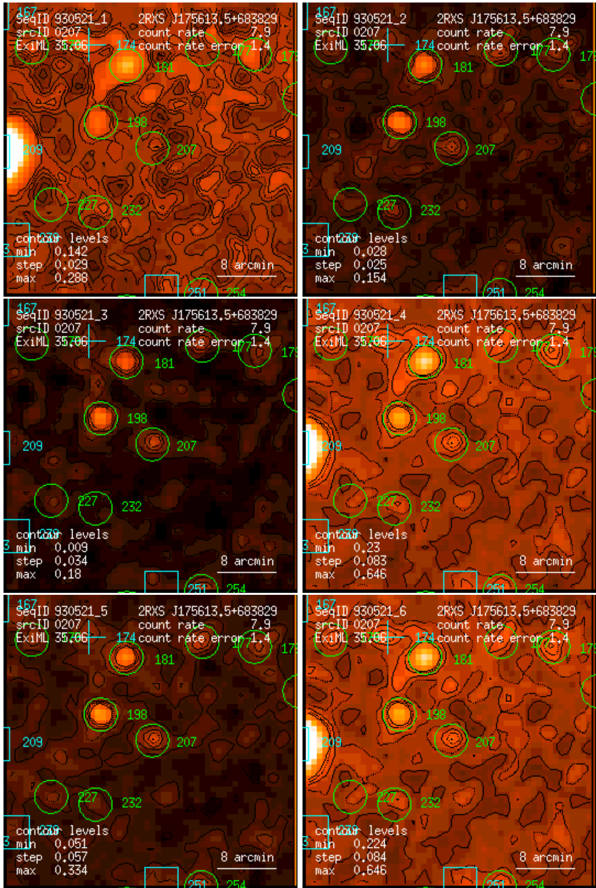
Figure 207: RASS 930521: detection 0207: band rate images, Gaussian filter: (1) PSPC channels 11 – 41, (2) 52 – 90, (3) 91 – 201, (4) 11 – 235, (5) 52 – 201, (6) 11 – 201. Broad band rates in counts/ks. Band rate contour levels in counts/ks/arcmin 2 .
