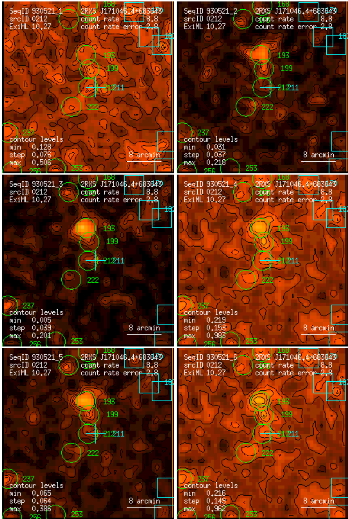
Figure 212: RASS 930521: detection 0212: band rate images, Gaussian filter: (1) PSPC channels 11 – 41, (2) 52 – 90, (3) 91 – 201, (4) 11 – 235, (5) 52 – 201, (6) 11 – 201. Broad band rates in counts/ks. Band rate contour levels in counts/ks/arcmin 2 .
